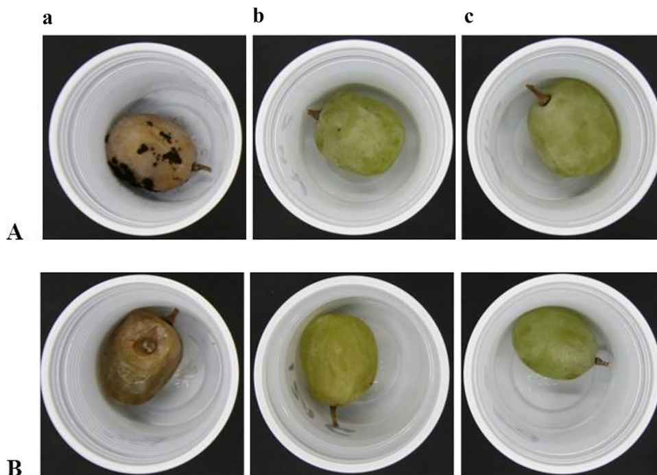
Fig. 6 Table grapes artificially contaminated with A. niger CECT 2805 (A) or B. cinerea CECT 20,973 (B) without LAB (a) or in the presence of F. fructosus AREP6 (b) or L. plantarum MEP3 (c) after 14 days of storage at 4 °C
