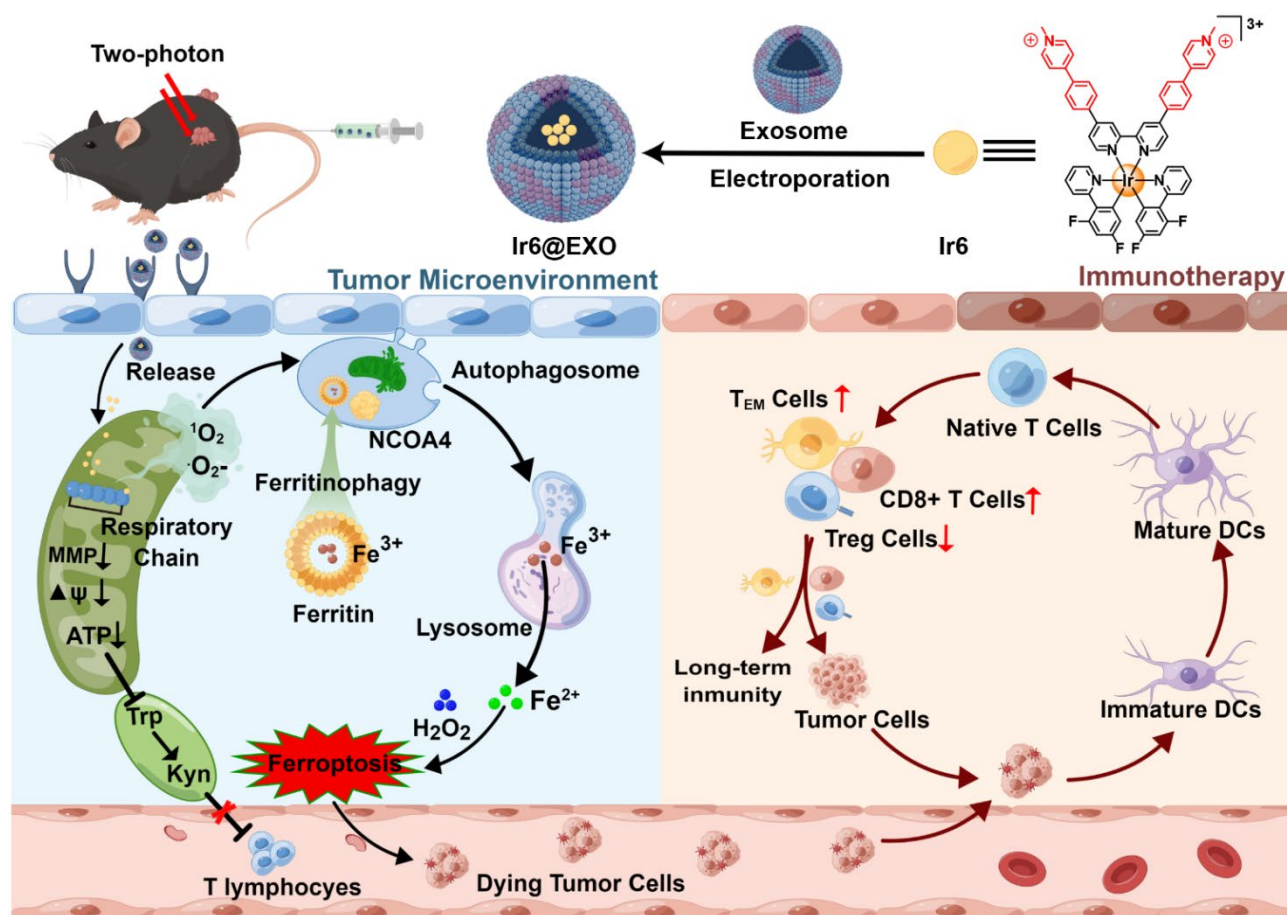
Scheme 1. Schematic view of the encapsulation within exosomes of Ir6 that induces mitochondrial ROS production upon two-photon irradiation, leading to the disruption of the mitochondrial respiratory chain and the induction of ferritinophagy-mediated immunogenic cell death.
