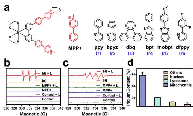
Figure 1. (a) Chemical structures of the Ir(III) photosensitizers Ir1–Ir6 and MPP+. (b) Electron spin resonance spectra of Ir6 and MPP+ upon incubation with the ^1\text{O}_2 -specific scavenger 2,2,6,6-tetramethylpiperidine in the dark or upon light irradiation (L). (c) Electron spin resonance spectra of Ir6 and MPP+ upon incubation with the scavenger 5,5-dimethyl-1-pyrroline-N-oxide in the dark or upon light irradiation (L). (d). The subcellular distribution of A375 cells upon incubation with Ir6 (10 \mu\text{M} ) for 6 h to determine the metal content inside the major organelles. L = two-photon laser irradiation at 720 nm, 40 mW, 120 s.
