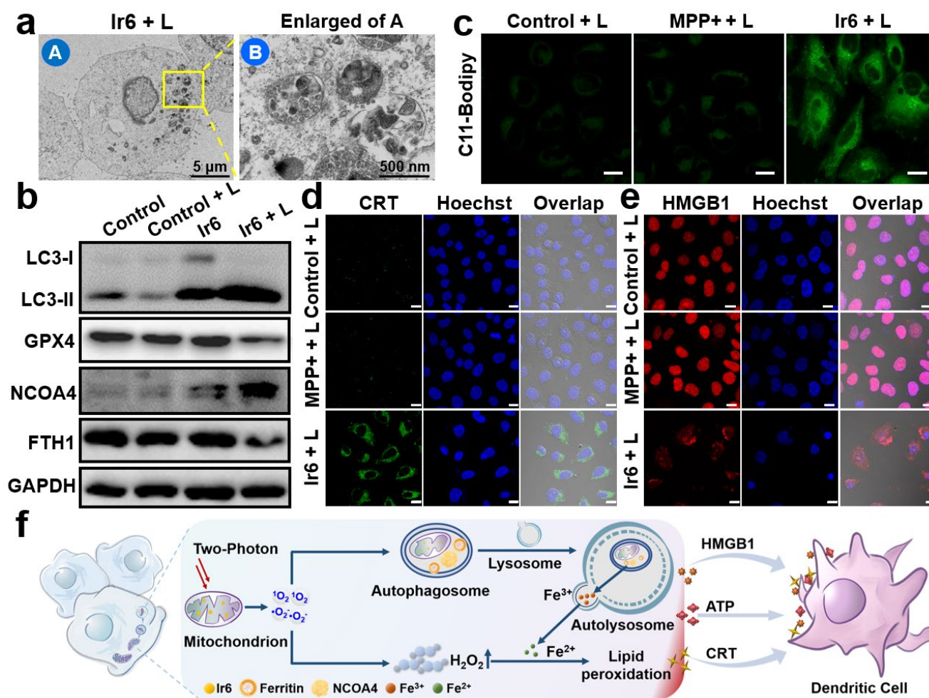
Figure 3. Cell death mechanism of Ir6 in A375 cells. (a) Representative transmission electron microscopy image of the autophagosomes of A375 cells upon treatment with Ir6 upon irradiation (L). (b) Western Blot analysis of the expression level of LC3-I, LC3-II, GPX4, NCOA4, and FTH1 of A375 cells upon treatment with Ir6 in the dark or irradiation (L). (c) CLSM of A375 cells incubated with the lipid peroxide-specific probe C11-Bodipy and treated with MPP+ or Ir6 upon irradiation (L). Scale bar = 20 \mu m. Immunofluorescence CLSM of A375 cells incubated with (d) CRT-specific antibody and (e) HMGB1 protein-specific antibody and treated with MPP+ or Ir6 upon irradiation (L). Scale bar = 20 \mu m. (f) Proposed cell death mechanism of ferritinophagy and immunogenic cell death by Ir6 upon irradiation. Concentration: Ir6 (10 \mu M), MPP+ (100 \mu M). L = two-photon laser irradiation at 720 nm, 40 mW, 120 s.
