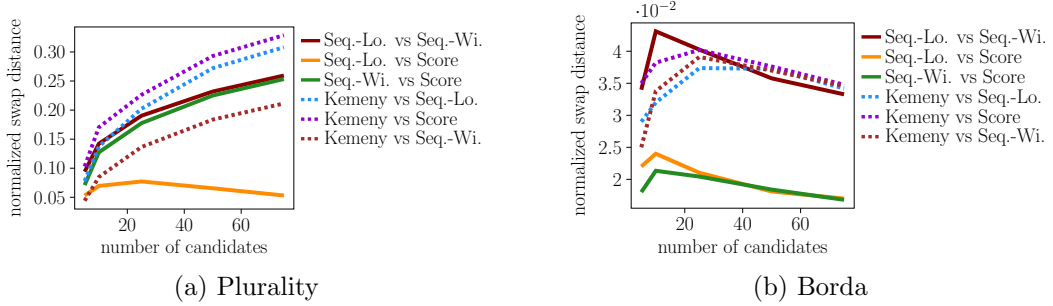
Figure 6: Pairwise average normalized swap distance between the Kemeny ranking and rankings produced by our three scoring-based methods on profiles sampled from Mallows model with \text{norm-}\phi = 0.8 with 100 voters and a varying number of candidates.
