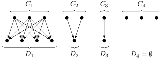
Figure 9: A bilevel graph as described in Lemma C.5.
