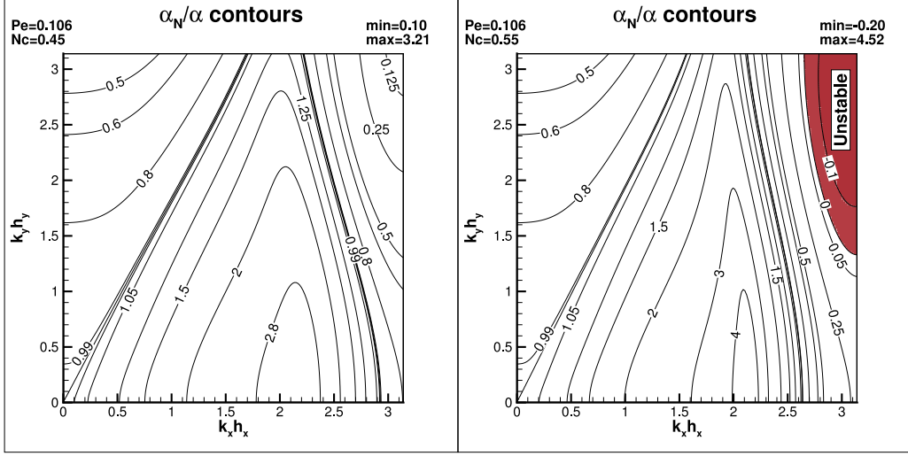
Fig. 38. Numerical diffusion- \frac{\alpha_N}{\alpha} contours for the RK_4 -UD 3 -CD 2 scheme for the 2D CDE. The space time properties are indicated by the CFL ( Nc ) and Pe values with AR = 1 , \theta = 0^\circ , respectively.
