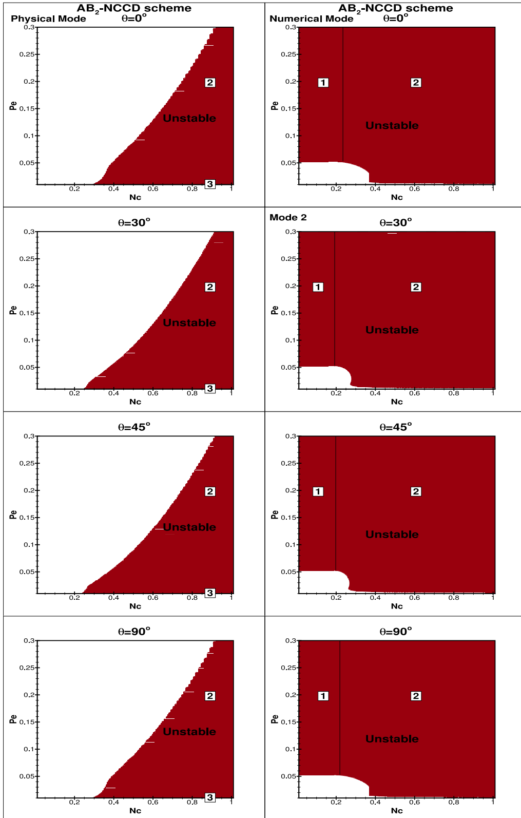
Fig. 40. Influence of wave propagation angle \theta of the 2D CDE on the critical Peclet number for AB_2 - NCCD scheme with grid aspect ratio AR = 1 . Unstable regions are indicated by the dark patches in the (Nc, Pe) -plane. Left frames correspond to the physical mode while right frames correspond to the numerical mode of AB_2 .
