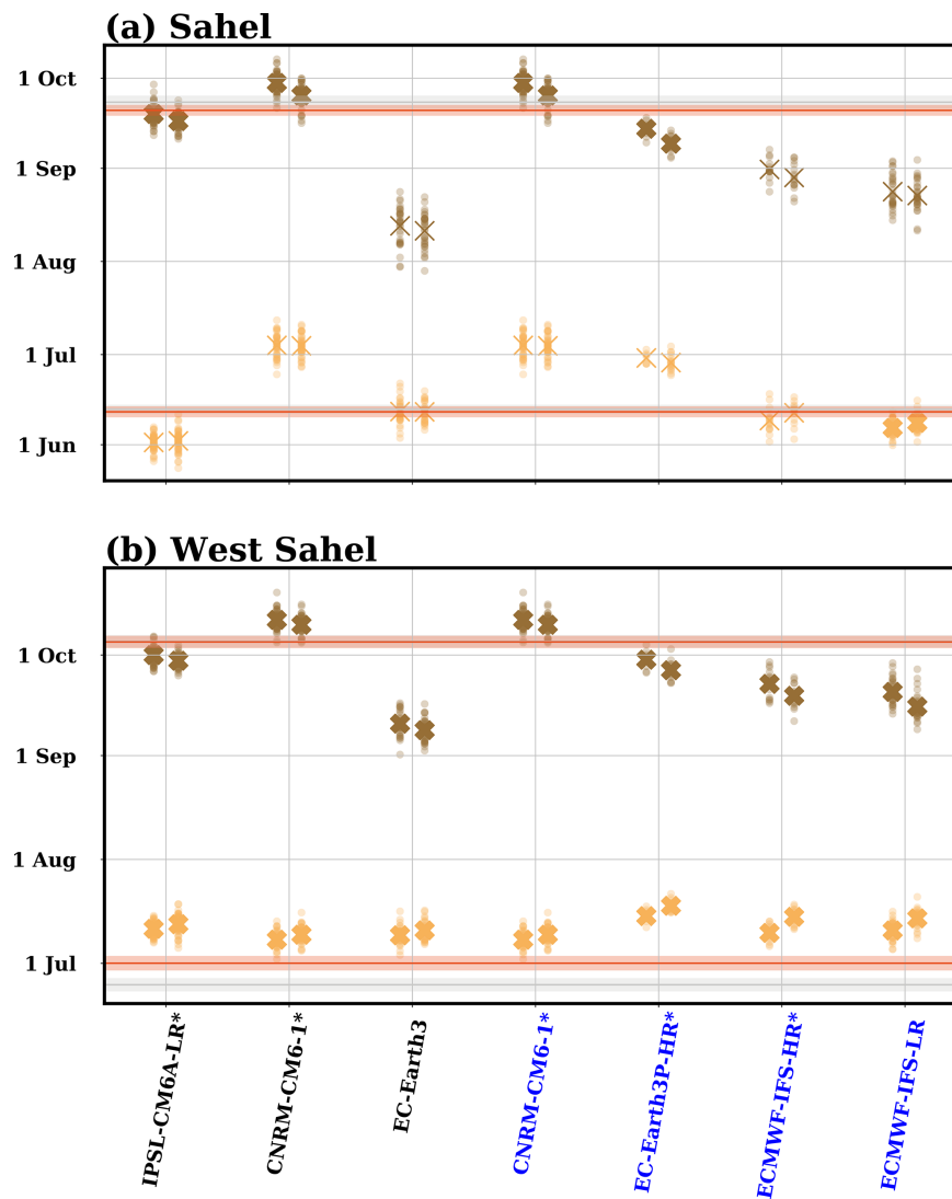
Figure 6. Dates for the monsoon onset (orange) and demise (brown) in models averaged over the (a) Sahel (defined as the area 10–20° N and 10° W–10° E; see red box in Fig. 1c and d) and (b) westernmost Sahel (10–20° N, 17–10° W, after removal of the area west of the line connecting the points 12° N–17° W and 10° N–15° W; see purple box in Fig. 1c and d) for the simulations. PRIMAVERA simulations are marked blue in the model labels. The values for the AMV+ simulation are shown slightly to the left of the corresponding axis for each model, while the ones for the AMV– simulation are located to the right. Small circles show the averages for 10 years in each ensemble member, while big crosses show the values averaged over all ensemble members. Crosses are bold if the AMV+ minus AMV– differences are statistically significant ( p < 0.05 ). Values of monsoon onset and demise are shown for the rainfall estimates obtained from MSWEPv280 (red line; climatology 1979–2020) and CHIRPS (gray line; climatology 1981–2021). Shading indicates the standard deviation of 10-year running mean values (so that they can be compared with 10-year means for each ensemble). The asterisk in the names of the models indicates that the AMV+ minus AMV– difference in the length of the monsoon is statistically significant ( p < 0.05 ) when averaged over the Sahel box. The differences in the length of the season for the westernmost Sahel box are all statistically significant ( p < 0.05 ).
