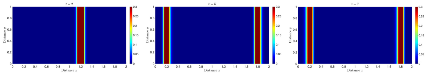
Fig. 5.1. Reference solutions obtained for the wave reflections in a rectangular domain using the FVM on the reference mesh with 23855 elements and 120037 nodes at three different times t = 2, 5 and 7 .
