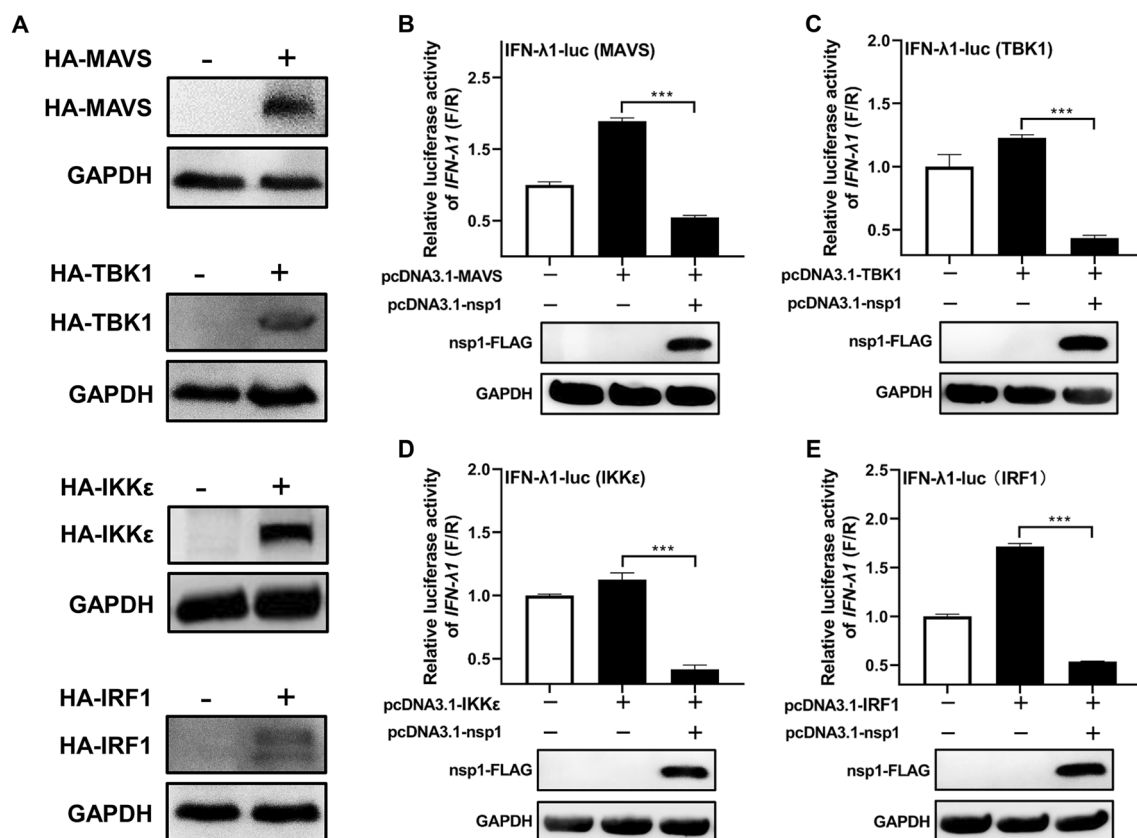
Figure 4 Inhibition of the RLR signaling pathway by SADS-CoV nsp1. A Expression of MAVS, TBK1, IKK \epsilon , and IRF1 in IPI-FX cells detected by Western blot. B–E SADS-CoV nsp1 inhibits the RLR signaling pathway. IPI-FX cells were co-transfected with nsp1, along with expression plasmids for MAVS ( B ), TBK1 ( C ), IKK \epsilon ( D ), or IRF1 ( E ), as well as IFN- \lambda 1-luc and pRL-TK at a ratio of 1:1:0.1:0.01 for 24 h. Cell lysates were prepared, and luciferase activity was measured. Data are represented as the mean \pm SD of three replicates. *** P < 0.001 .
