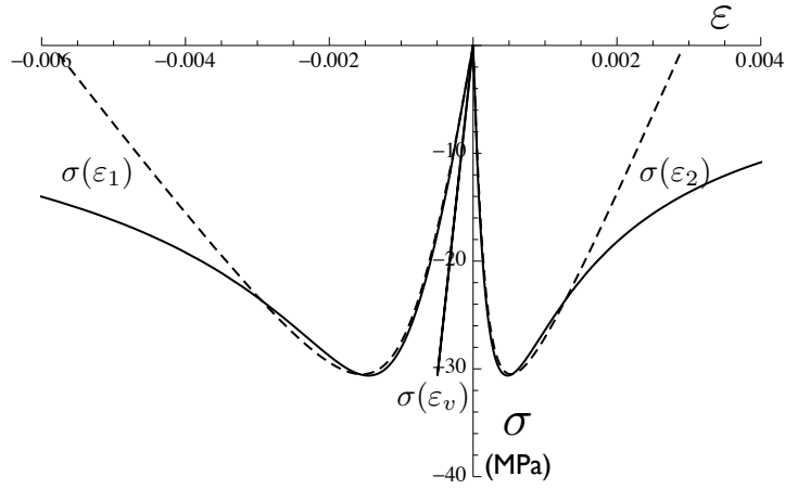
Figure 11. Response of proposed anisotropic damage model in compression (dashed line: initial anisotropic damage model).
