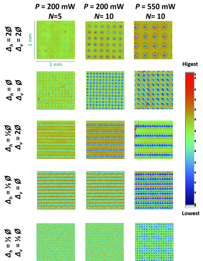
Fig. 2. Interferometric imaging of the textured surface treated by laser ablation. Each image has the same scale: 1 mm \times 1 mm. The horizontal beam lag, \Delta_h , the vertical beam lag, \Delta_v , the power density, P , and the number of pulses are modified to obtain a range of different roughness.
