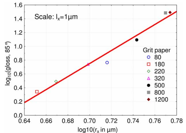
FIG. 11. The brightness versus the fractal radius curvature estimated at the scale of 1 \mu\text{m} for all polished surfaces with different paper indexes (80, 180, 220, 320, 500, 800, and 1,200). [Color figure can be viewed in the online issue, which is available at wileyonlinelibrary.com .]
