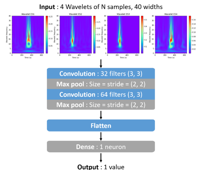
Figure 8. Hyperparameters of the CNN model giving the lowest reproducible uncertainty.
