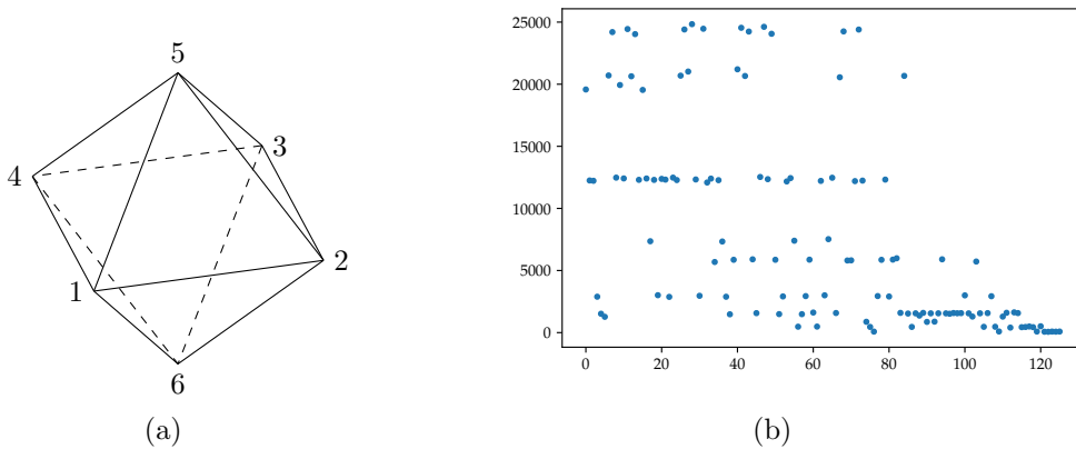
Figure 5: (a) A double tetrahedron or a simple triangulation of the sphere. (b) The number of passages in each paths for the random walk on the triangulation of the sphere. The paths are numbered, on the x-axis, by order of appearance. The y-axis contains the number of passages for each path during the first 10^6 steps.
