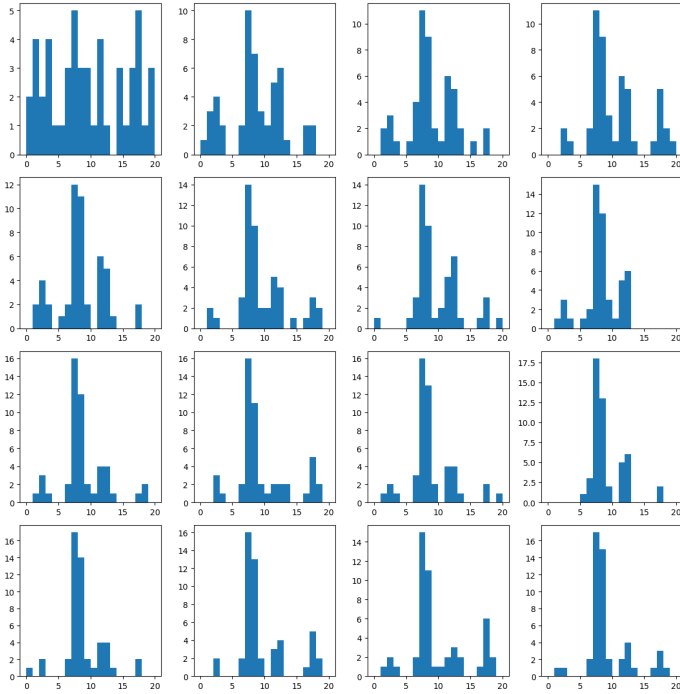
Figure 10: \|\hat{\rho}_t - \mathbb{1}_{\{7\}}\|_{L^2(\ell)} (1st generator)
