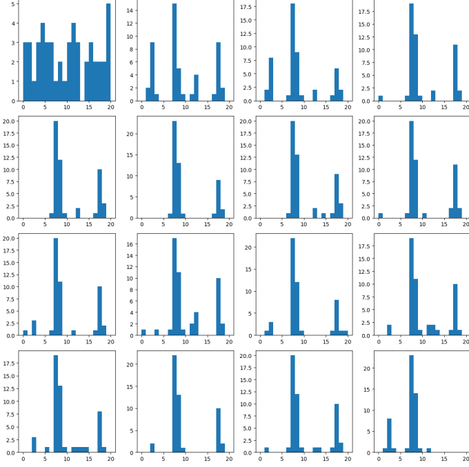
Figure 4: Empirical measure over time (1st generator)
