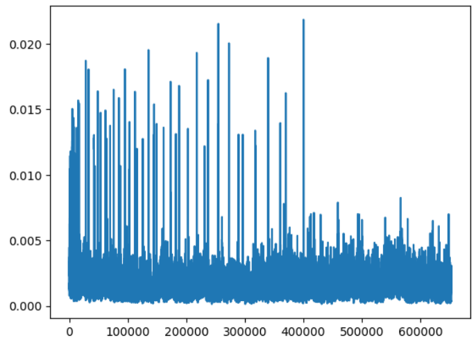
Figure 7: \|\hat{\rho}_t - \nu_t\|_{\mathbb{L}^2(\ell)} (2nd generator)
