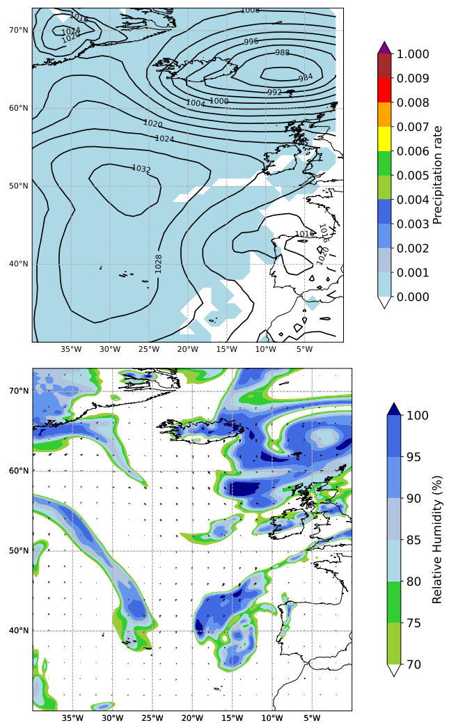
FIG. 2. Upper panel: MSLP and precipitation rate from the GFS analysis on 18 June 2022 at midday (12:00). Lower panel: The 850-hPa map of relative humidity.
