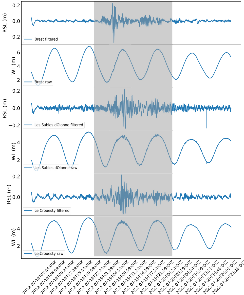
FIG. 16. De-tided and high-pass filtered (Butterworth) records of the event of 19 July 2022 at Brest, Les Sables-d'Olonne, and Le Croesty. The bottom plot of each panel shows the raw observed sea water level at the tide gauge. Data are recorded every minute. The shaded region highlights the time of the event.
