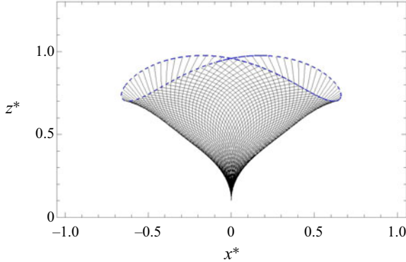
Figure 3. Beating pattern of the straight filament in the case with F_t^* = 40 , n = 1 and Re = 0.2 . The blue dashed line represents the filament-tip trajectory.
