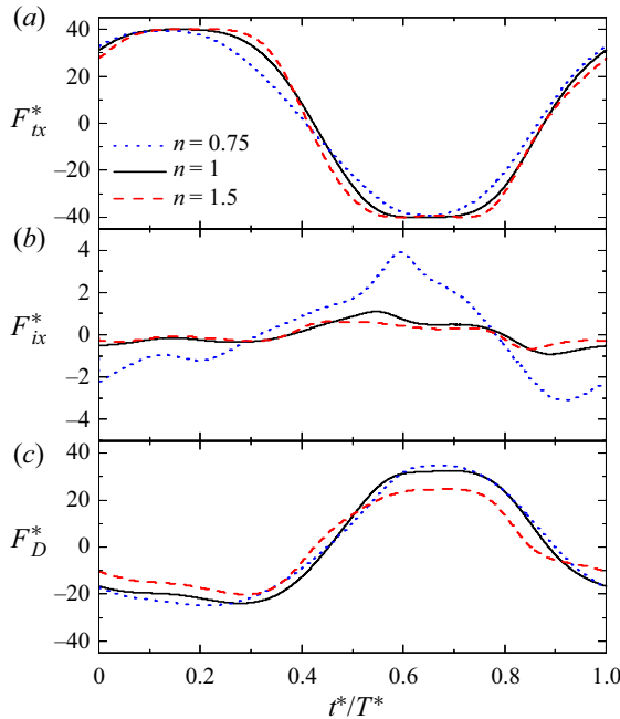
Figure 12. Time histories of (a) the x -component follower force ( F_{lx}^* ), (b) the x -component inertial force at the filament tip ( F_{ix}^* ) and (c) the drag force ( F_D^* ) in the cases with n = 0.75, 1 and 1.5 when Re = 0.2 and F_t^* = 40 .
