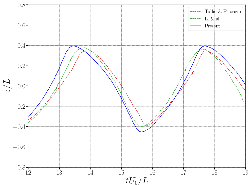
Fig. 14. Trailing edge position w.r.t time.
