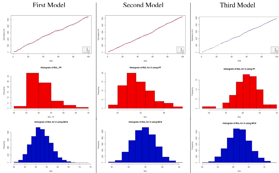
Fig. 5. System state estimation (top), Histogram of system's RUL using the third method (midst) and using Monte Carlo Simulations (bottom) for the different models, at t = 100 .
