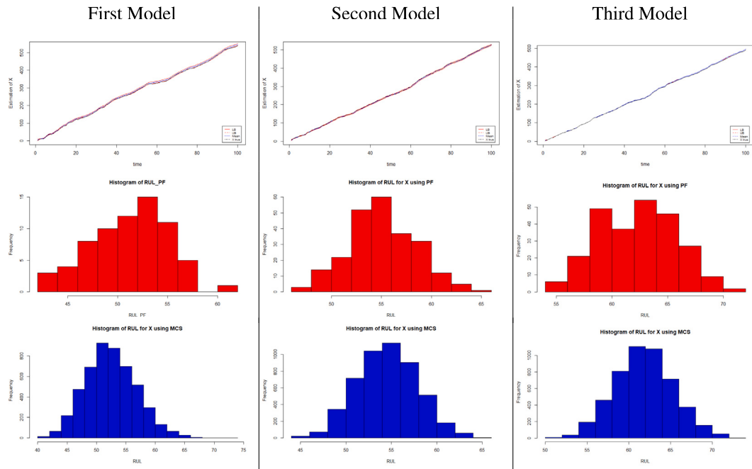
Fig. 4. System state estimation (top), Histogram of system's RUL using the second method (midst) and using Monte Carlo Simulations (bottom) for the different models, at t = 100 .
