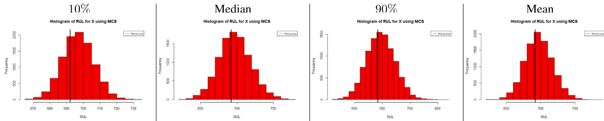
Fig. 11. Impact of the uncertainty around \hat{\sigma}_X on RUL's Histograms, for the first case.
