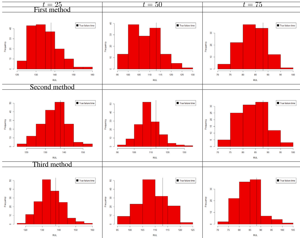
Fig. 6. RUL's histograms of the system with model W-W for different prognosis times.
