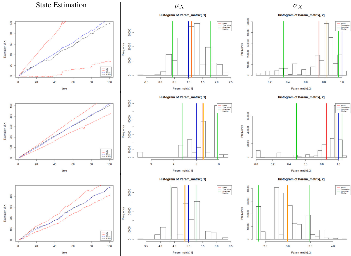
Fig. 8. State estimation for system's degradation(left panel) and histogram of \hat{\mu}_X (middle panel) and \hat{\sigma}_X n (right panel) for the different cases.
