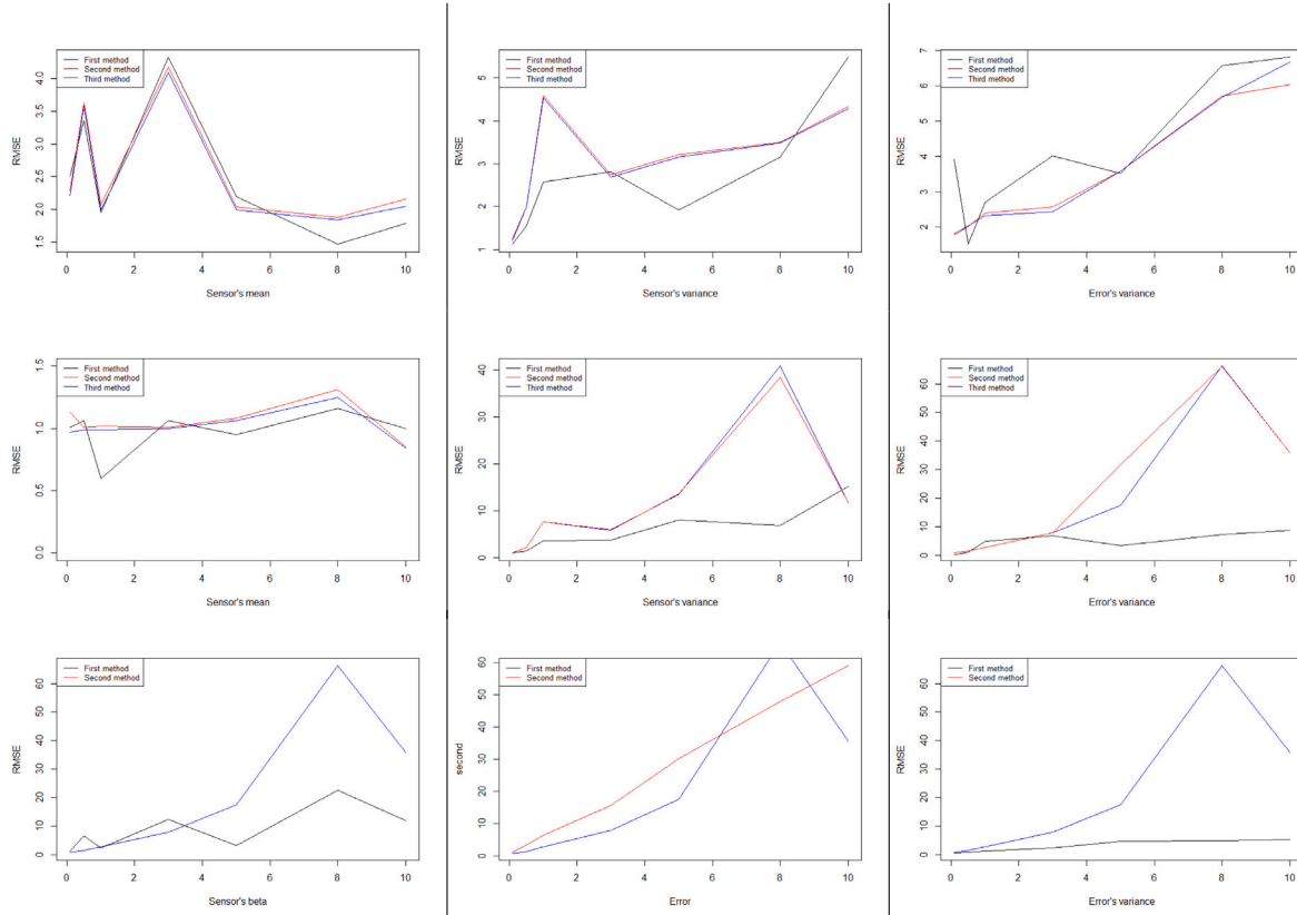
Fig. 2. System state estimation by the three methods for the three different case: first case (top), second case (midst), third case (bottom), at t = 100 , while varying the sensor's degradation parameters (left and midst) and the error \epsilon variance (right).
