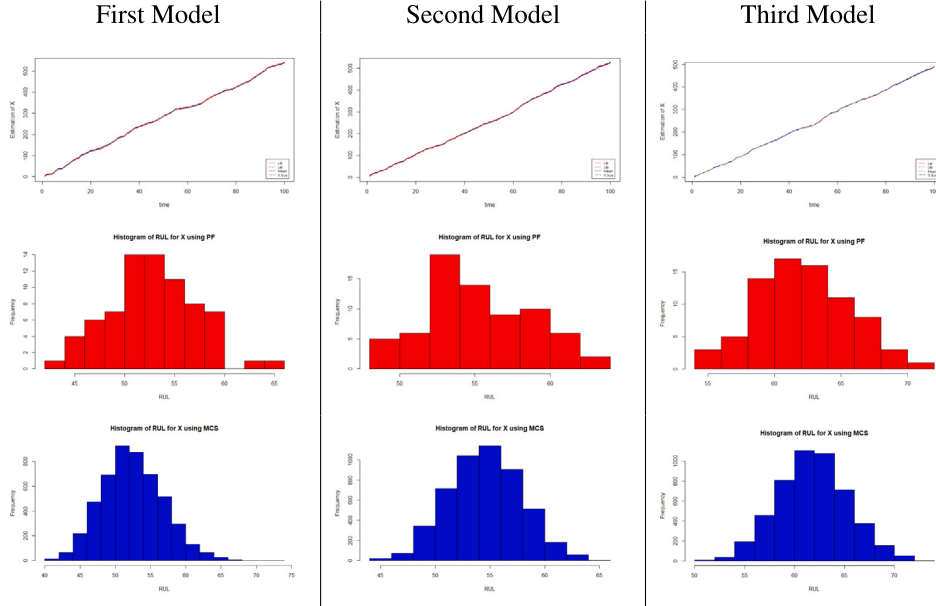
Fig. 3. System state estimation (top), Histogram of system's RUL using the first method (midst) and using Monte Carlo Simulations (bottom) for the different models, at t = 100 .
