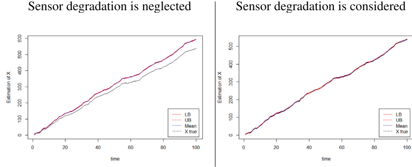
Fig. 1. Estimation of the system degradation at t = 100 .
