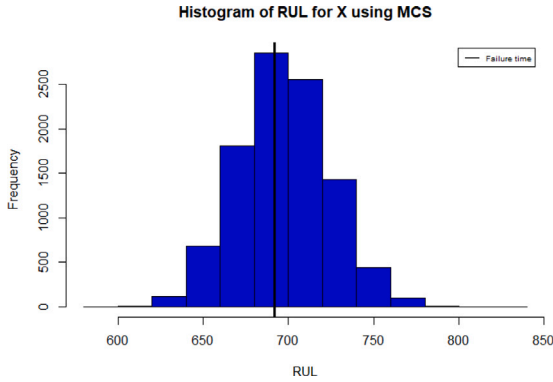
Fig. 9. RUL's histogram while using true parameters.
