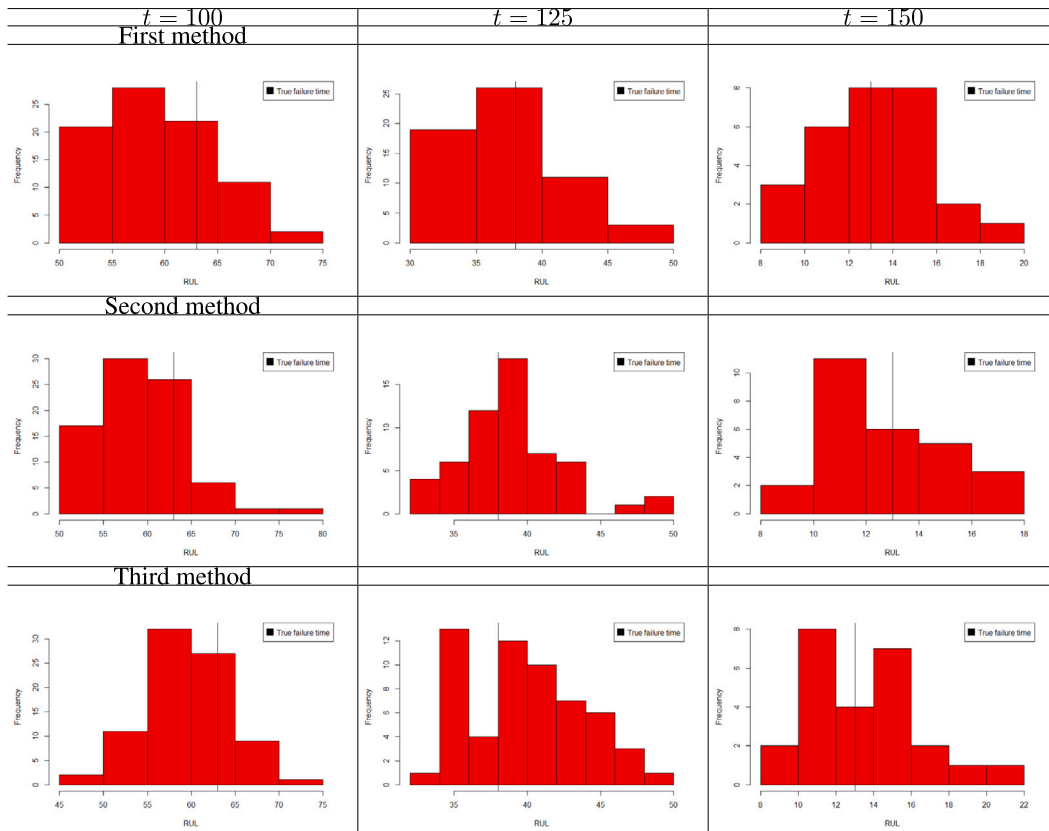
Fig. 7. RUL's histograms of the system with model W-W for different prognosis times.
