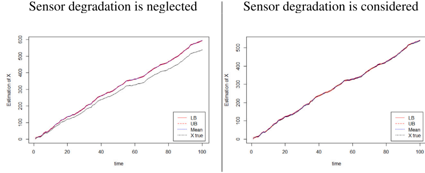
Fig. 1. Estimation of the system degradation at t = 100 .
