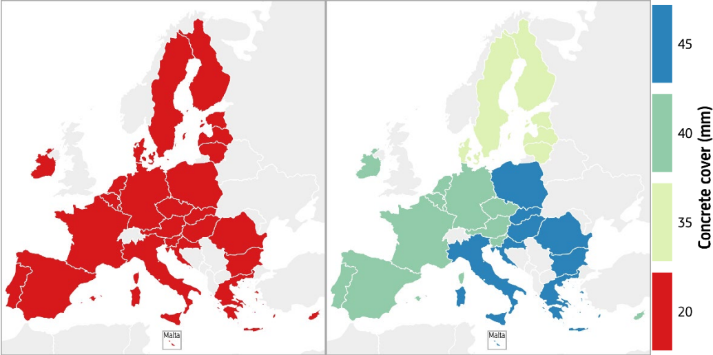
Figure 23. Concrete cover, c_t (mm), adopted for the 27 Member States; left: old buildings, right: recent buildings (Dimova et al. 2023).
