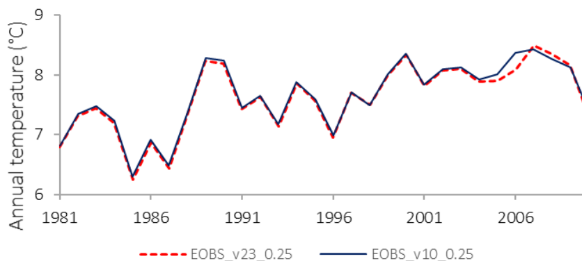
Figure 12. Evolution of annual mean temperature derived from E-OBSv10.0 and E-OBSv23.1 over 1981-2010.
