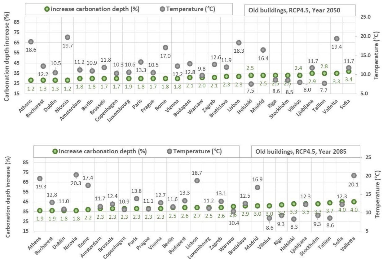
Figure 28. Percentage of increase of carbonation depth in EU-27 capital cities for old buildings , absolute temperature for a given year and temperature variation relative to the reference scenario.
