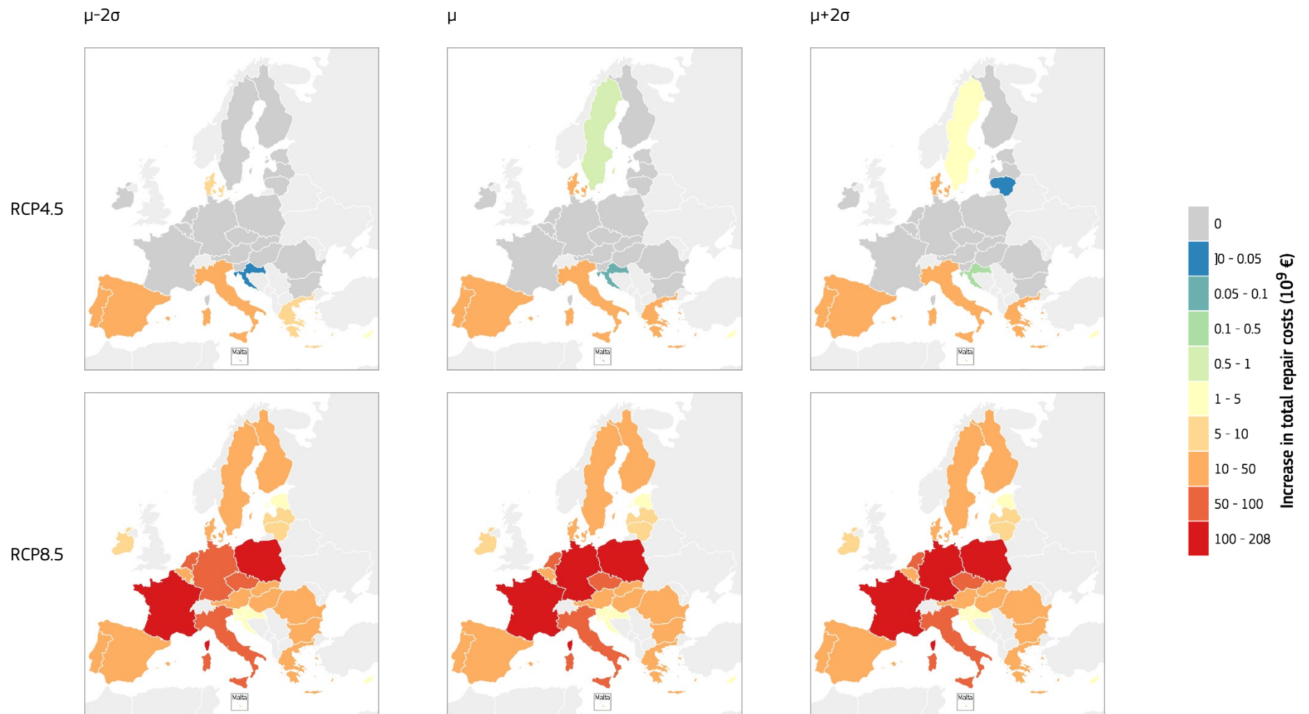
Figure 37. Total repair costs (10 9 €) due to climate change induced carbonation for the RC building stock (old buildings) of the EU-27 Member States by the year 2100.
