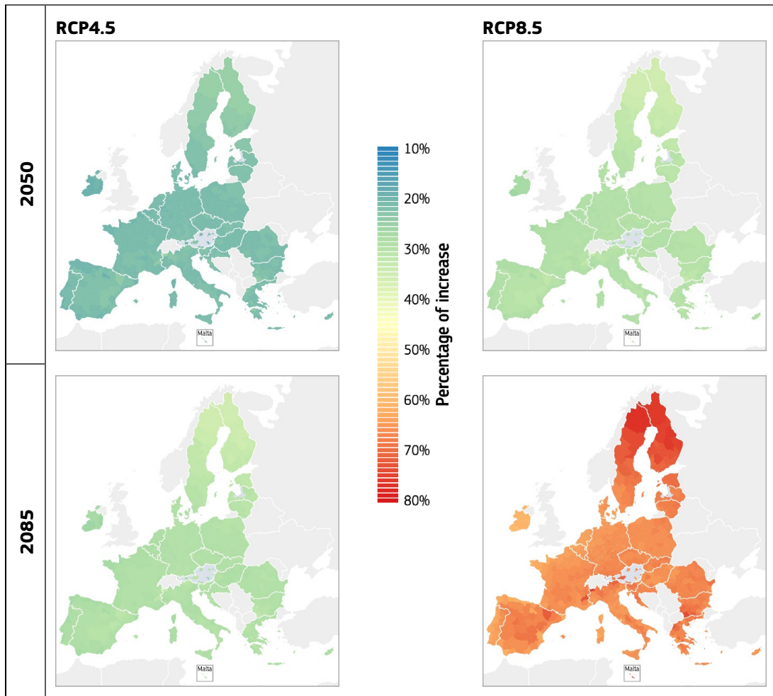
Figure 32. Percentage of increase of carbonation depth in EU-27 Member States for the RC building stock for the years 2050 (top) and 2085 (bottom) due to two climate change scenarios with respect to two control scenarios; left: RCP4.5 scenario, right RCP8.5 scenario.
