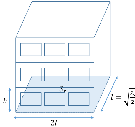
Figure 8. Idealized reinforced concrete building for the estimation of the exposed building surface façades.
