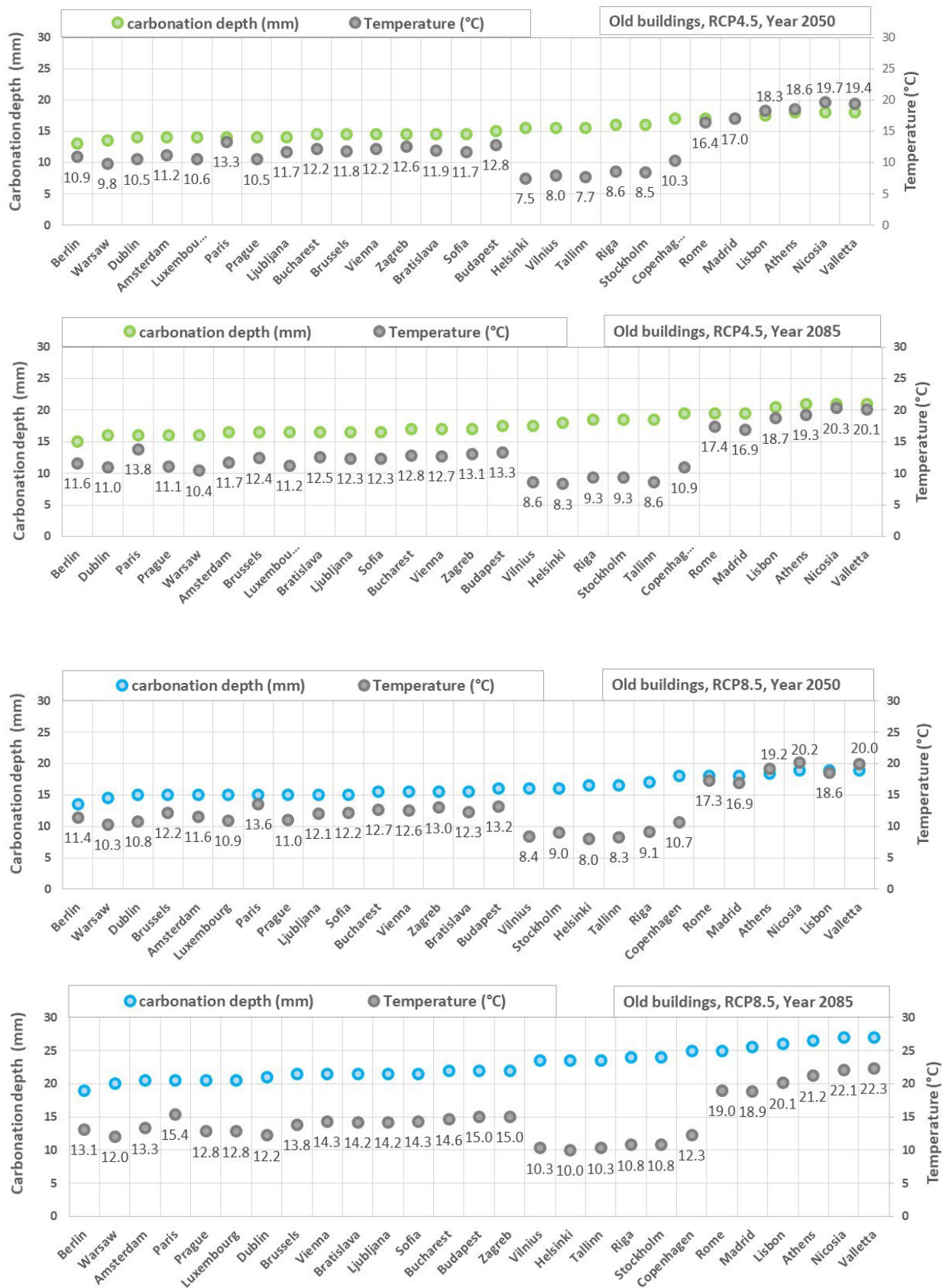
Figure 30. Absolute increase of carbonation depth in EU-27 capital cities for old buildings , absolute temperature for a given year and temperature variation relative to the reference scenario.
