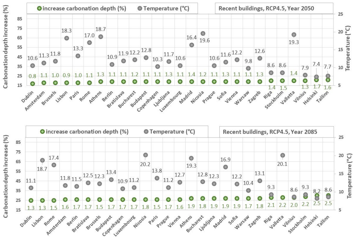
Figure 29. Percentage of increase of carbonation depth in EU-27 capital cities for recent buildings , absolute temperature for a given year and temperature variation relative to the reference scenario.
