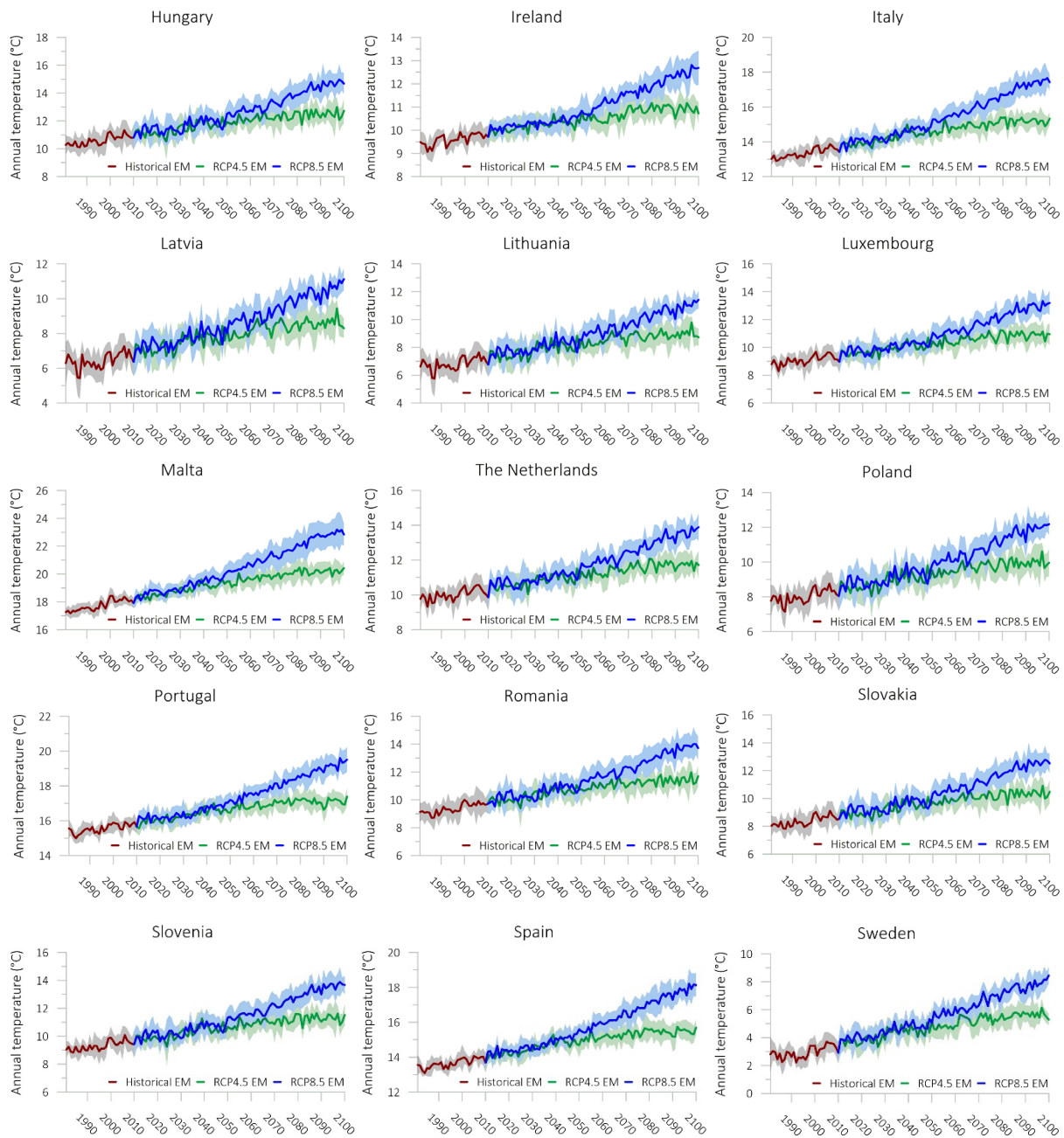
Figure 20. Trend of annual temperature at country level (part 2). Shaded areas represent the inter-model variability assessed as \pm\sigma .
