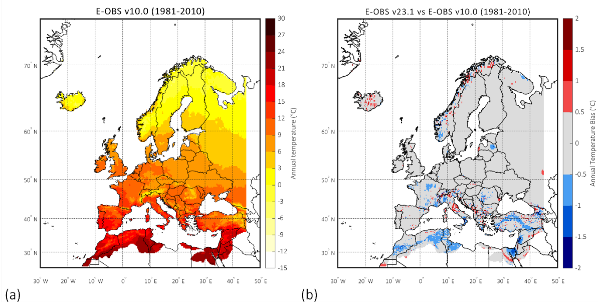
Figure 10. Map of annual temperature provided by E-OBSv10.0 over 1981-2010 (a); bias of annual temperature in-between E-OBS v10.0 and E-OBS v23.1 over the same period (b). Source: Developed by authors.
