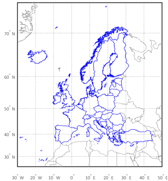
Figure 13. Delimitation of NUTSO Country (blue line). This area identifies in this work the European domain. Source: Developed by authors.
