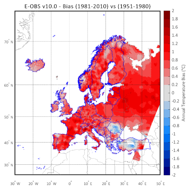
Figure 14. Map of variation of annual temperature given by E-OBS v10.0 over 1981-2010 against 1951-1980. Source: Developed by authors.
