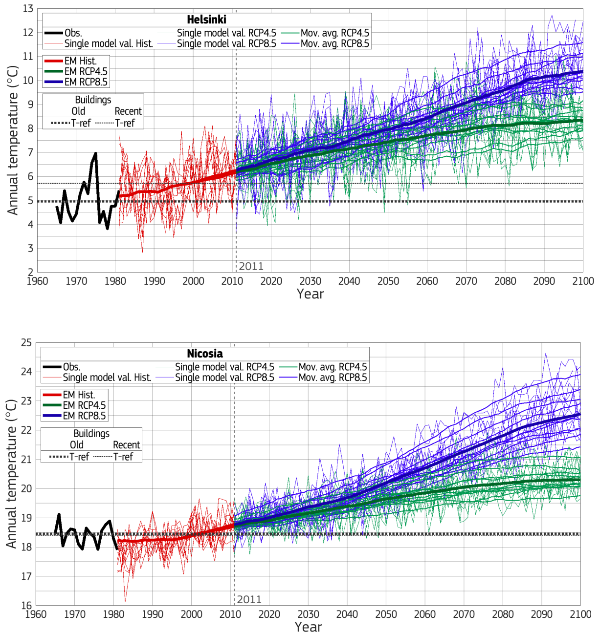
Figure 21. Trend of annual temperature in Helsinki (top figure) and Nicosia (bottom figure), observations, historical and projections scenarios.
