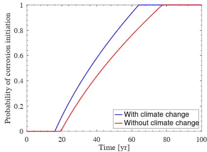
Figure 5. Probability of corrosion initiation over the time for two scenarios: with and without climate change.
