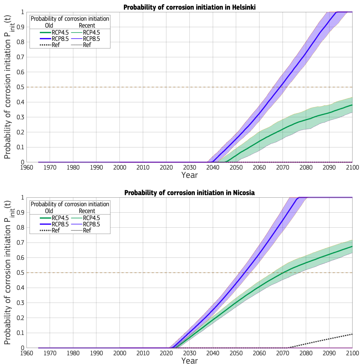
Figure 33. Probability of corrosion initiation in Helsinki (top figure) and Nicosia (bottom figure) for two climate change scenarios, RCP4.5 and RCP8.5 initiated in 2011, and two classes of buildings, old and recent buildings; Shaded areas are derived from the temperature inter-model variability and assessed between \pm 2\sigma .
