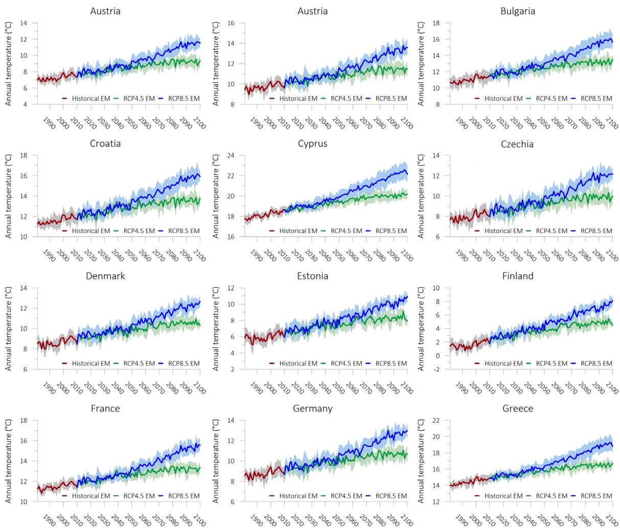
Figure 19. Trend of annual temperature at country level (part 1). Shaded areas represent the inter-model variability assessed as \pm\sigma .
