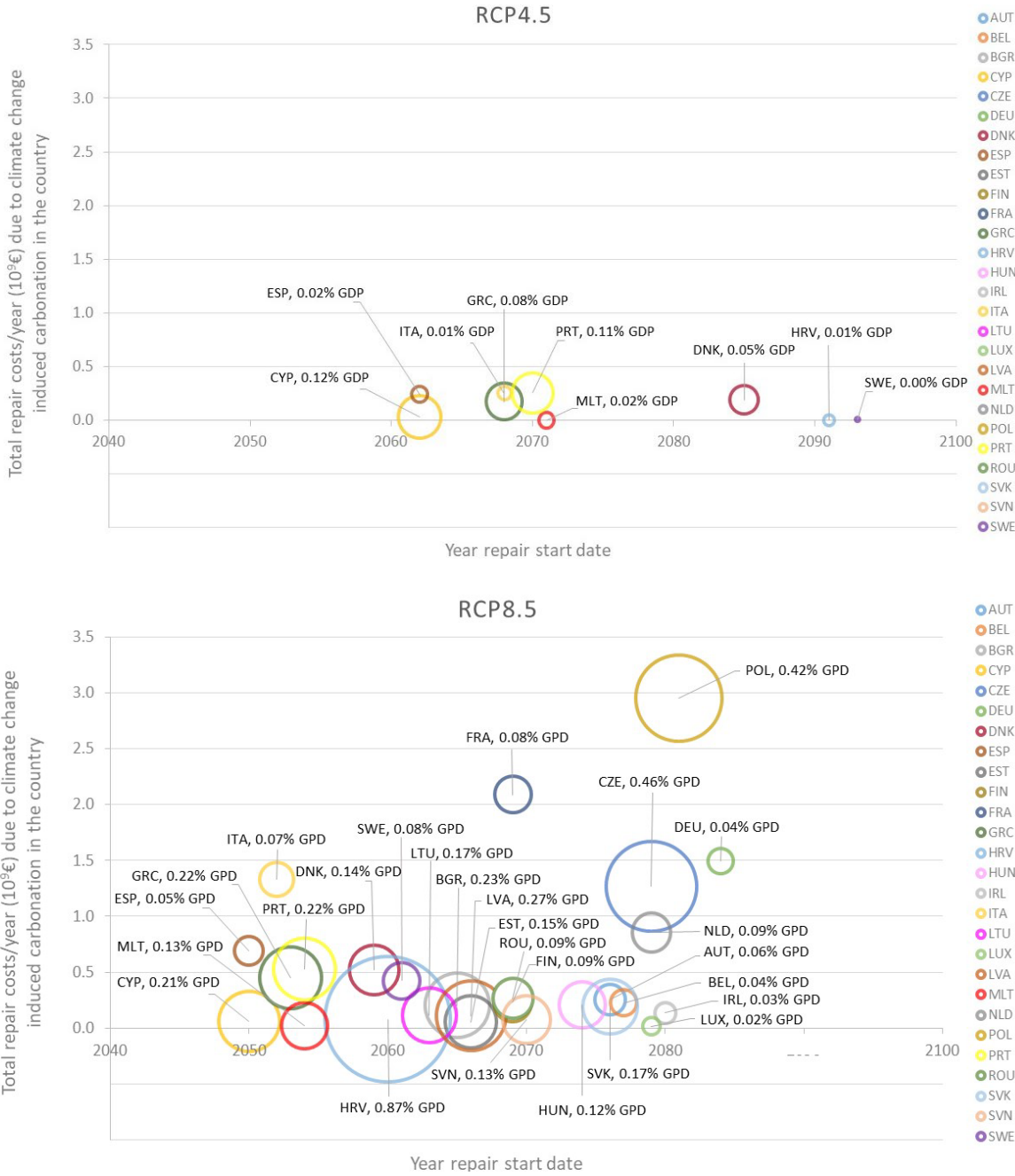
Figure 38. Total repair costs by year (billion euro, B€) and percentage impact on GDP by country, analysed in relation to RCP4.5 and RCP8.5 scenarios.
