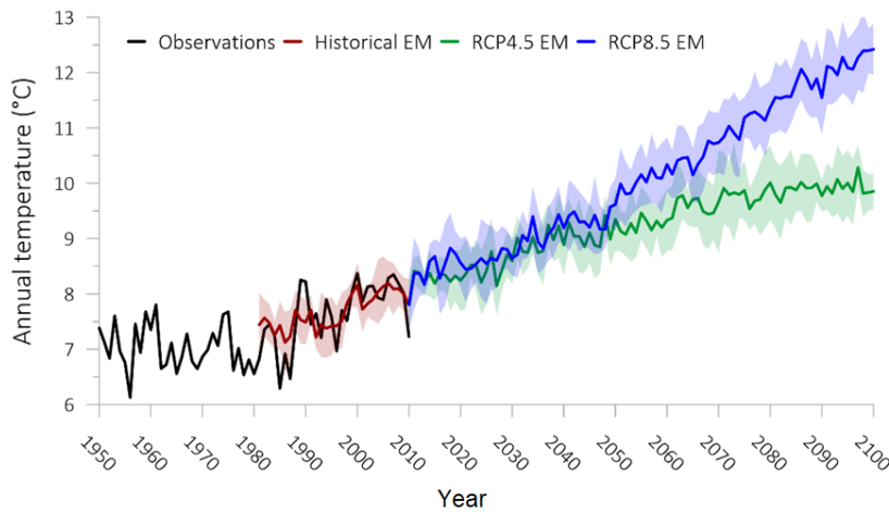
Figure 18. Trend of annual temperature over Europe. Shaded areas represent the inter-model variability assessed as \pm\sigma .
