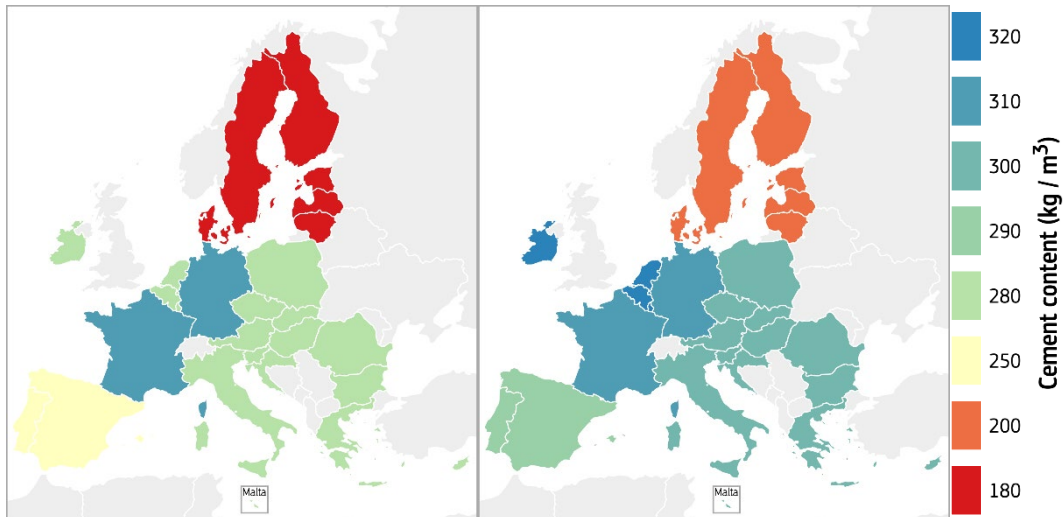
Figure 25. Cement content, C_e ( \text{kg}/\text{m}^3 ), adopted for the 27 Member States; left: old buildings, right: recent buildings.
