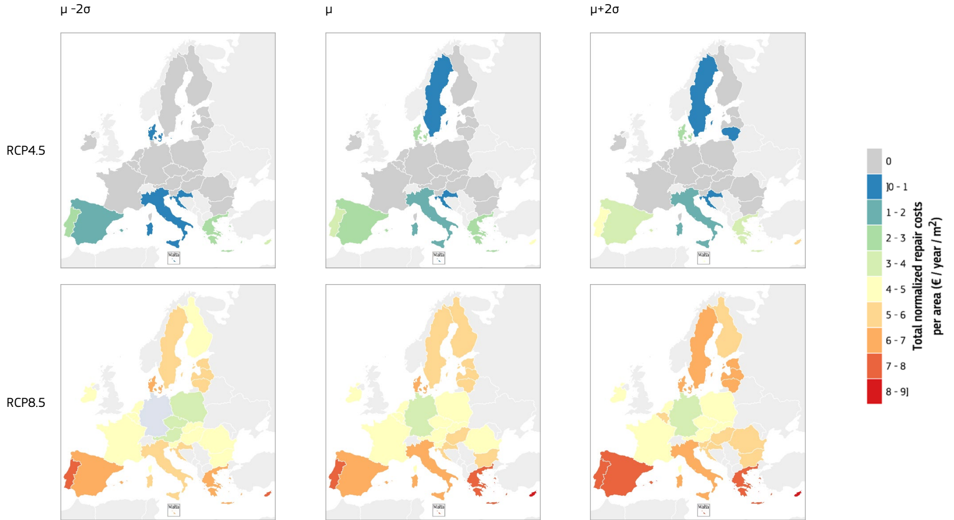
Figure 35. Total normalized repair costs per square meter and year (€/year m 2 ) for old RC buildings in the EU-27 Member States.
