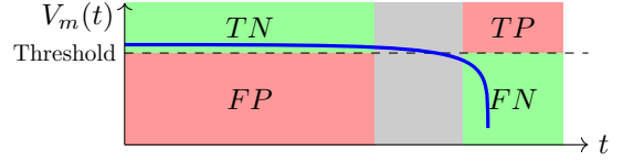
Fig. 2. Algorithm evaluation.
