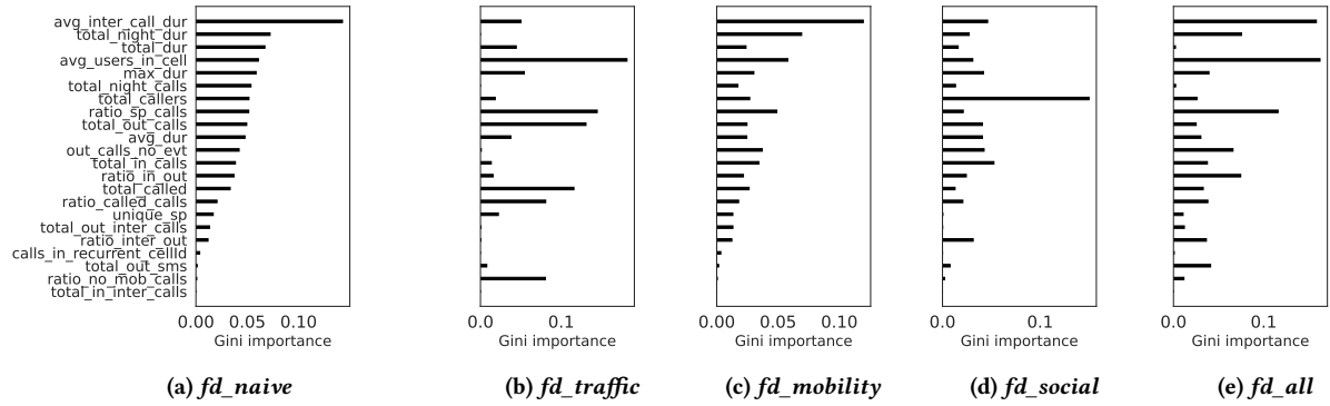
Figure 5: Average relative importance of detection features per fraud model, F^{T_o}(all) feature set, T_o=day .
