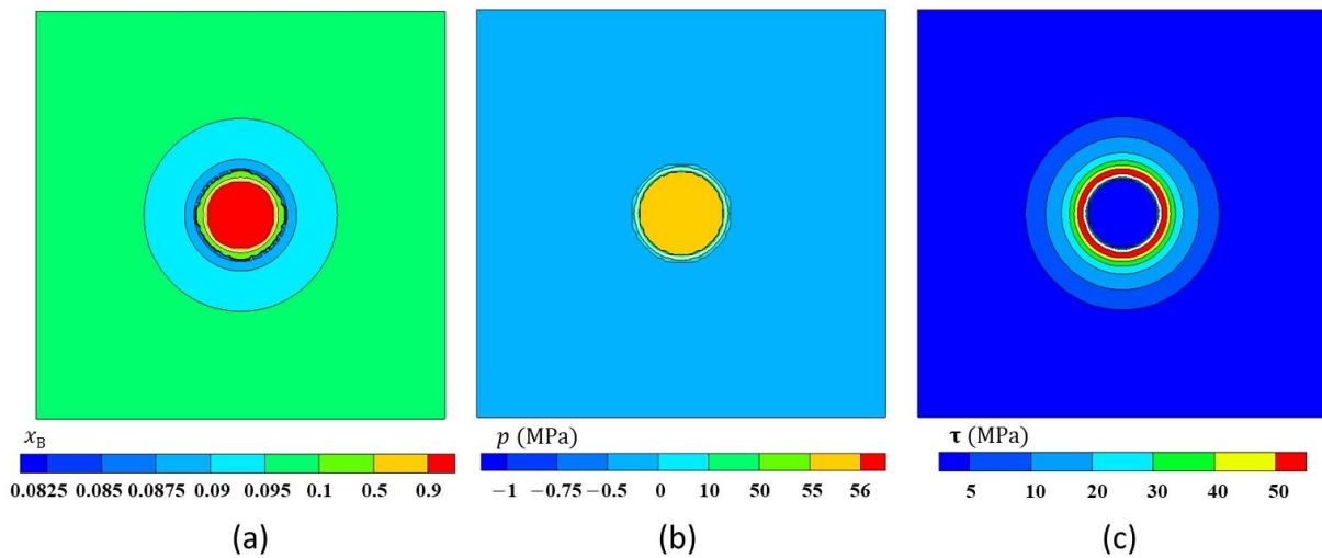
Figure 3. Maps within the three equivalent middle planes X = 0.5, Y = 0.5, and Z = 0.5 at dimensionless time t \cdot D/L^2 = 0.15 of (a) molar fraction of B-atoms; (b) pressure. Note that the positive value of pressure corresponds to compressive pressure, whereas negative value corresponds to tensile pressure.; (c) Normalized shear stress.
