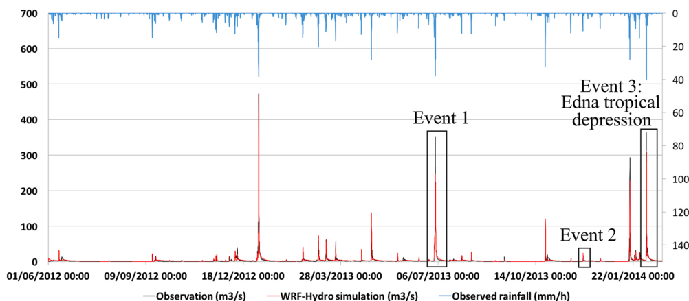
Fig. 5. WRF-Hydro simulated (red) and observed (black) hydrograph of Dumbéa Est watershed. Rainfall is plotted in blue along the top axis. Calibrations were carried out on the three events labeled as black boxes. Left axis for streamflow is in \text{m}^3\text{ s}^{-1} and right axis for rainfall is in \text{mm h}^{-1} .
