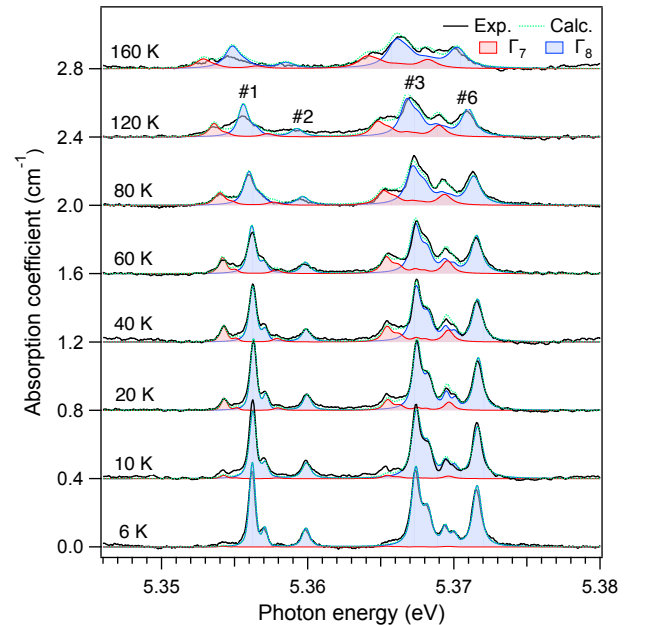
FIG. S2. (a) Absorption spectra of boron-doped diamond from 6 to 160 K. Measured spectra (black lines) are compared with the sum (dotted green lines), calculated for the transitions from the \Gamma_8 (blue lines) and \Gamma_7 (red lines) acceptor levels. Spectral broadening by the detection system was included in the calculation.
