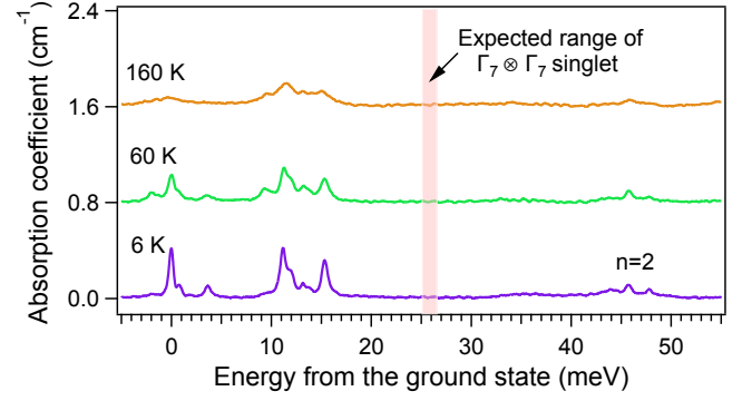
FIG. S3. Absorption spectra of boron-doped diamond obtained at different temperatures indicating the absence of transition to \Gamma_7 \otimes \Gamma_7 singlet. The n = 2 components correspond to excited quasiexciton states of the bound exciton [17].
