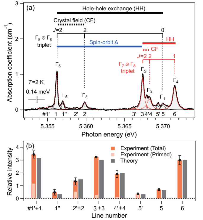
FIG. 4. (a) Higher-resolution absorption spectrum at 2 K (thick black line) fitted with the sum (dotted red line) of eleven Voigt functions, #1'–#6 (thin lines). The labels near the respective peaks represent the symmetry of the two-hole states. The brackets and horizontal bars at the top indicate two sets of triplets and the approximate size of the splittings, respectively. (b) Comparison of the experimental and theoretical absorption strengths. Orange bars with dots indicate the areal intensities of #1, #2, and #4 superposed on top of #1', #2', and #4', respectively. Thinner bars indicate intensities of primed peaks. The theory (gray bars) includes the electron-hole exchange effect for lines #1'–#2 and valley-orbit splitting for #5' and #5 (details in Sec. III of Supplemental Material [37]).
