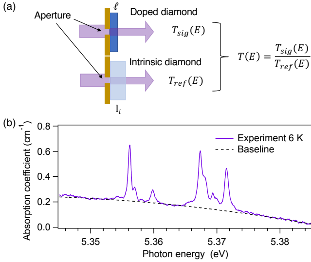
FIG. S1. (a) Schematic of measurement principle for transmission through boron-doped and intrinsic diamond samples. (b) Spectrum of -(1/\ell) \ln[\mathcal{T}(E)/\mathcal{T}_0] at 6 K (solid line) and the baseline B(E) (dashed line).
