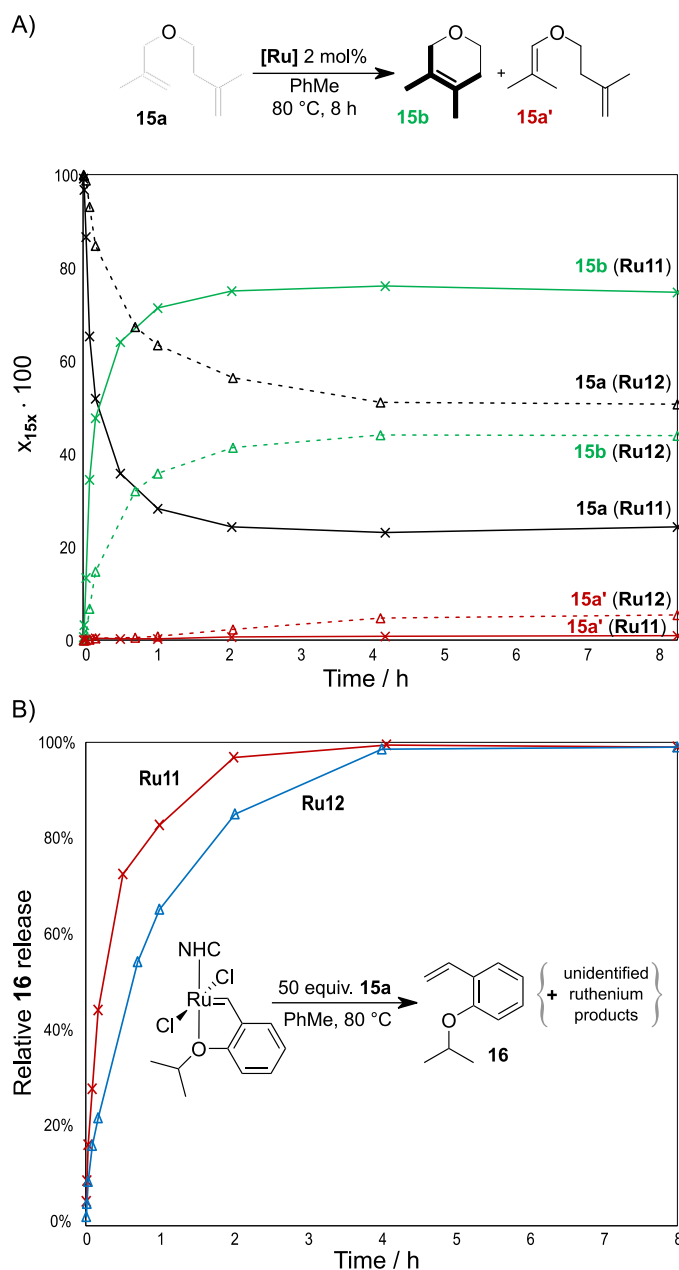
Figure 10. A) Reaction profile of substrate 15a RCM. B) o -isopropoxystyrene ( 16 ) release during RCM of diene 15a .
