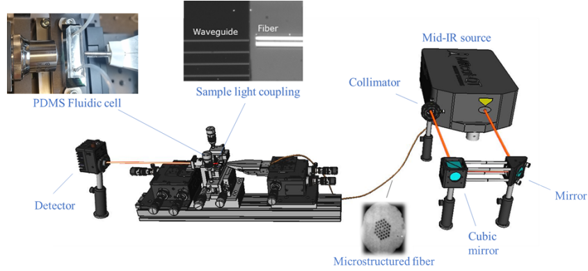
Fig. 4. Schematic diagram of the optical bench platform sensor.
