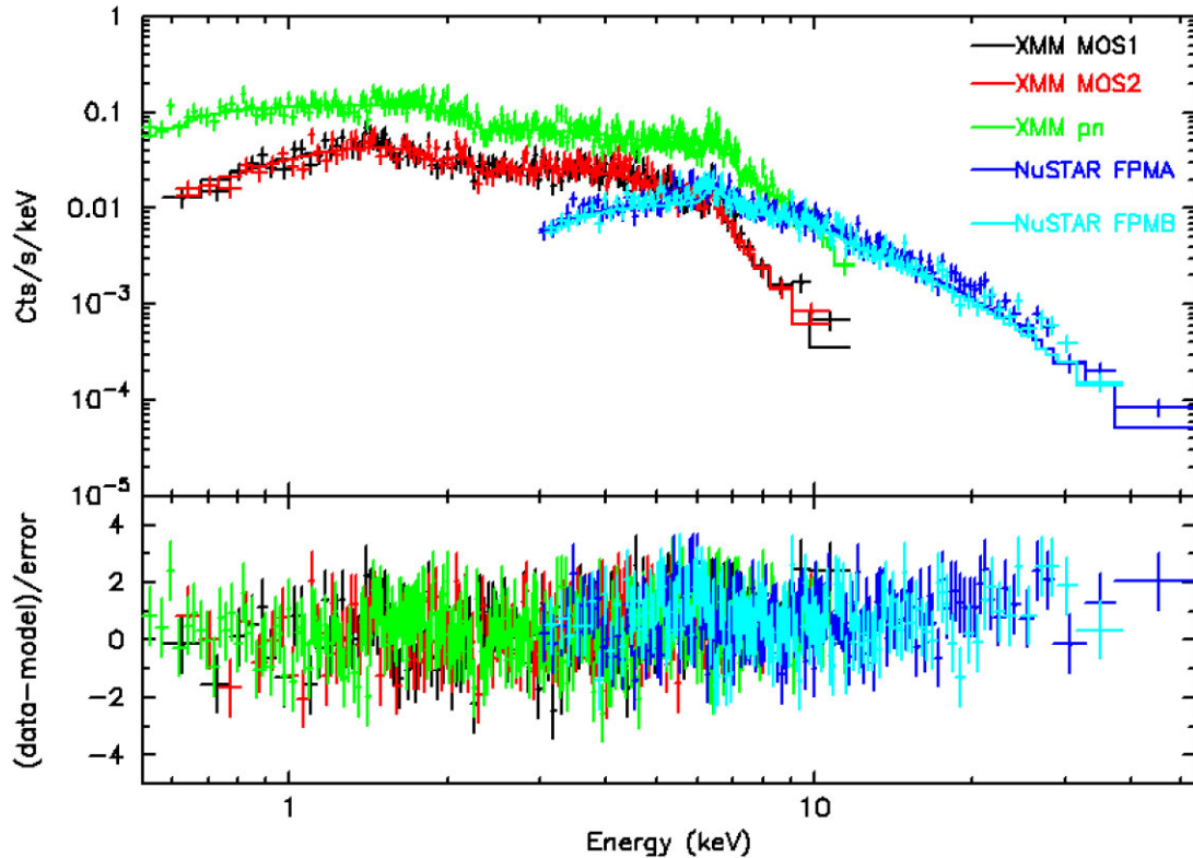
Figure 5. XMM-Newton and NuSTAR joint spectrum (with residuals) fit to the PSR model and three narrow Gaussians. The best-fitting parameters for this model are listed in Table 3.
