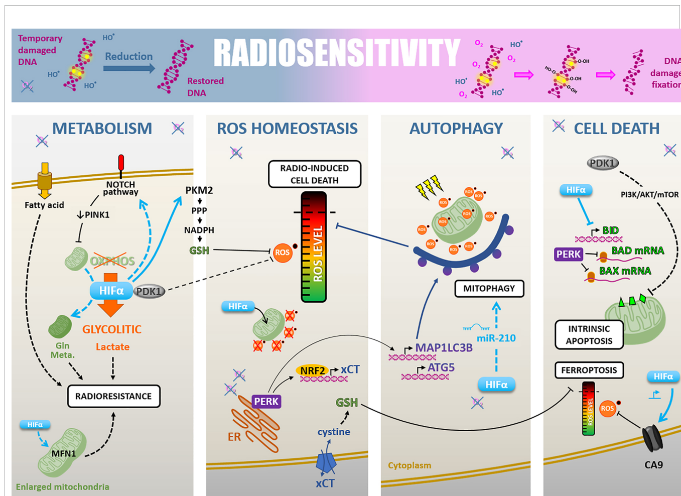
FIGURE 3 | Radiosensitivity. Cell-intrinsic radiosensitivity can be linked to the fixation of radiation-induced DNA damages in the presence of oxygen, whereas a hypoxic environment favors the reduction of DNA radicals and return to a restored DNA (upper part). Hypoxia also impacts radiosensitivity through different cellular adaptations. i) The cell metabolism modifications, mainly PDK1-mediated glycolytic switch leading to lactate production, but also fatty acid uptake, NOTCH-dependent mitochondrial glutamine metabolism increase, and mitochondria fusion. ii) The ROS homeostasis is maintained under the critical level by PDK1 increase, HIF \alpha -mediated GSH regeneration, HIF \alpha translocation to mitochondria leading to their ROS production decrease, and PERK-mediated xCT expression promoting GSH synthesis. iii) Induction of HIF \alpha - and PERK-mediated autophagy of ROS-productive damaged mitochondria. iii) The cell death regulation through a HIF \alpha -, PDK1- and PERK-mediated inhibition of antiapoptosis modulators BID, BAD, and BAX, and a HIF \alpha -induced CA9 expression decreasing ROS level and inhibiting ferroptosis.
