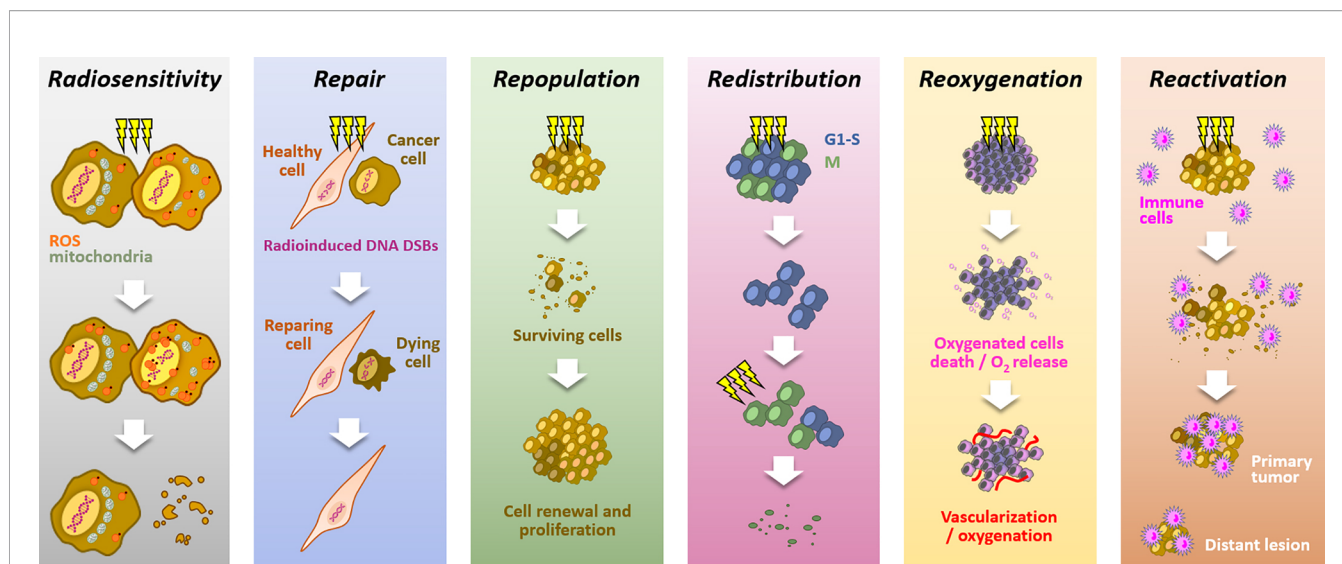
FIGURE 1 | The six “Rs” dictating the response to radiotherapy. Radiotherapy response depends on six parameters: Radiosensitivity , refers to the cell-intrinsic mechanisms (e.g., metabolic adaption, ROS detoxification), explaining differences in cell responses to irradiations; Repair , refers to the cell capacity to survive by repairing radio-induced damages (particularly DSBs), in theory, more characteristic of healthy cells; Repopulation , refers to the tumor cells capacity to grow following a radiotherapy fraction; Redistribution , refers to the progression of cancer cells from radioresistant cell cycle phases (i.e., G1/S) toward more radiosensitive phases (i.e., G2/M), between radiotherapy fractions; Reoxygenation , refers to the oxygen level recovery following irradiation, due to well-oxygenated cells death and tumor vascularization; Reactivation , refers to the triggering of a systemic anti-tumor immune response following irradiation-induced immunogenic cell deaths.
