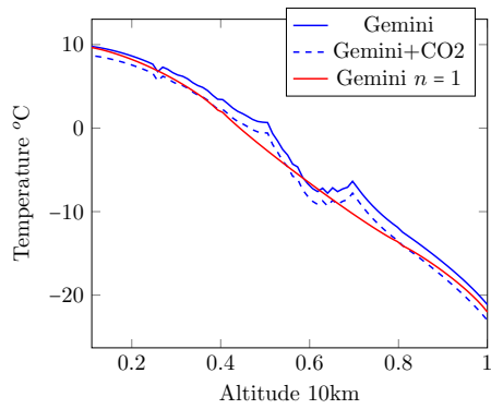
Figure 7: Case 1 (top) & Case 2 (bottom). Temperature versus altitude. The dashed curve is computed with \kappa_1 to account for \text{CO}_2 .
