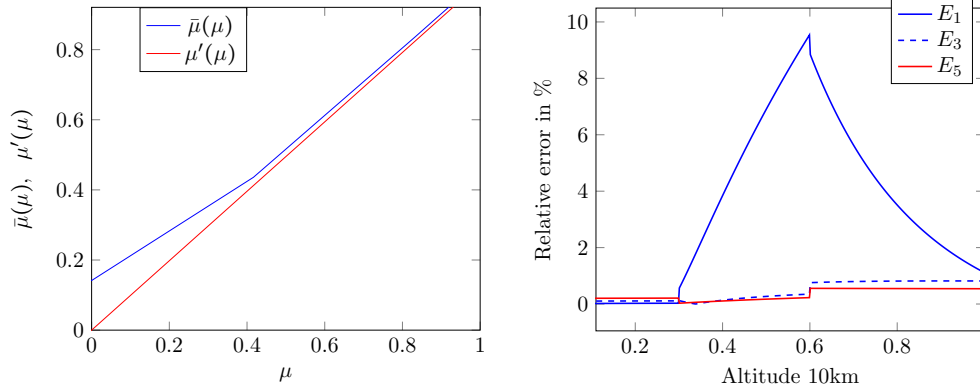
Figure 1: Difference between \mu'(\mu) and \bar{\mu}(\mu) (see (5.1)) when n_{z'}/n_z = 0.99 .
