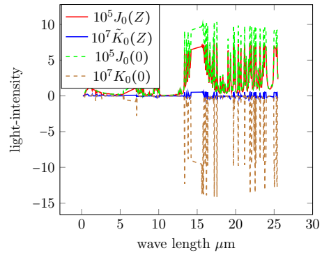
Figure 8: Case 1 (top) & Case 2 (bottom) with \kappa . Total light intensity J_0 and polarized K_0 versus wave length at ground level and altitude 10km.
