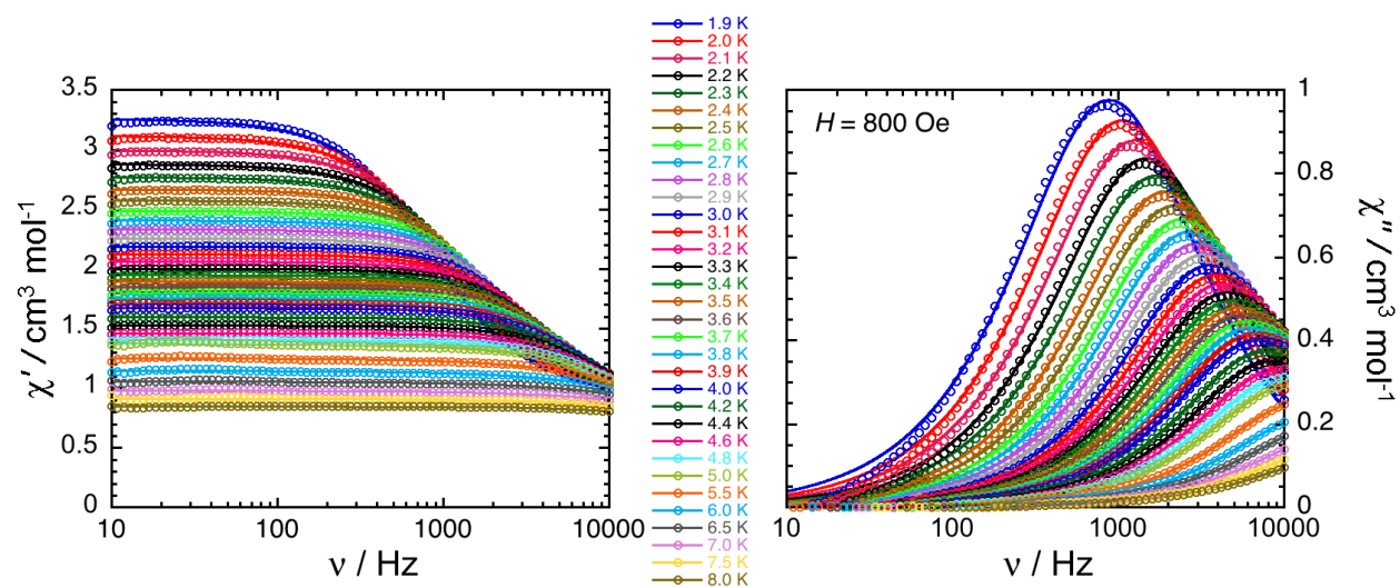
Supplementary Figure 13. Frequency dependence of the in-phase ( \chi' ; left) and out-of-phase ( \chi'' ; right) components of the ac susceptibility for \text{Eu}\{\text{N}(\text{SiMePh}_2)_2\}_2 ( 1 ) between 1.9 and 8 K for ac frequencies between 10 Hz and 10 kHz under an applied static field of 800 Oe. Solid lines represent the fits to the generalized Debye model.
