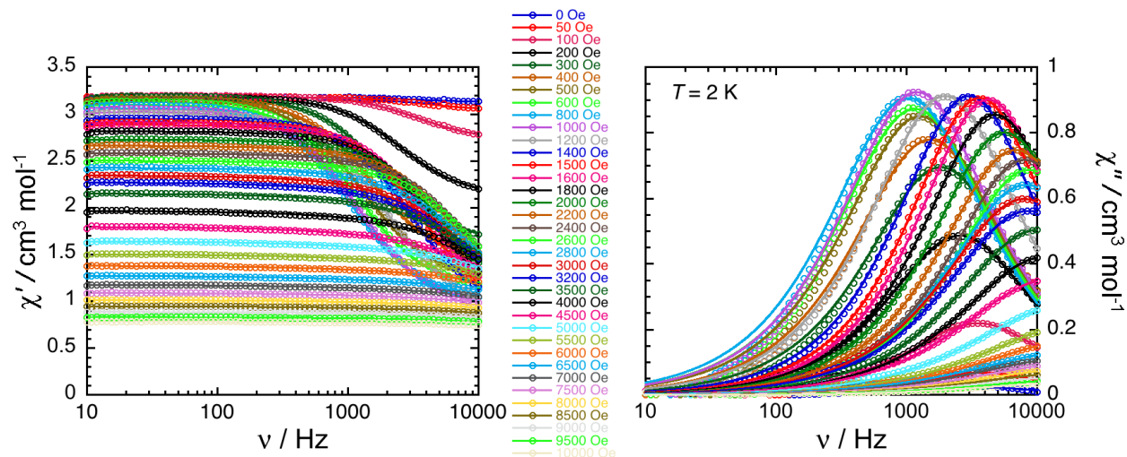
Supplementary Figure 9. Frequency dependence of the in-phase ( \chi' ; left) and out-of-phase ( \chi'' ; right) components of the ac susceptibility for \text{Eu}\{\text{N}(\text{SiMePh}_2)_2\}_2 ( 1 ) between 0 and 10 kOe for ac frequencies between 10 Hz and 10 kHz at 2 K. Solid lines represent the fits to the generalized Debye model.
