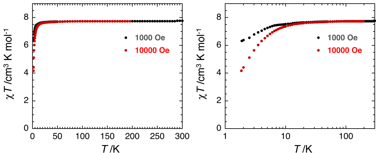
Supplementary Figure 6. Linear (left) and semi-logarithm (right) \chi T versus T plots at 1 kOe and 10 kOe between 1.85 and 300 K for \text{Eu}\{\text{N}(\text{SiMePh}_2)_2\}_2 ( 1 ) ( \chi is defined as the magnetic susceptibility equal to M/H per mole of complex). At 1 kOe, the 300 K and 1.85 K \chi T products are respectively 7.8 and 6.3 \text{cm}^3 \text{K/mol} for \text{Eu}\{\text{N}(\text{SiMePh}_2)_2\}_2 ( 1 ).
