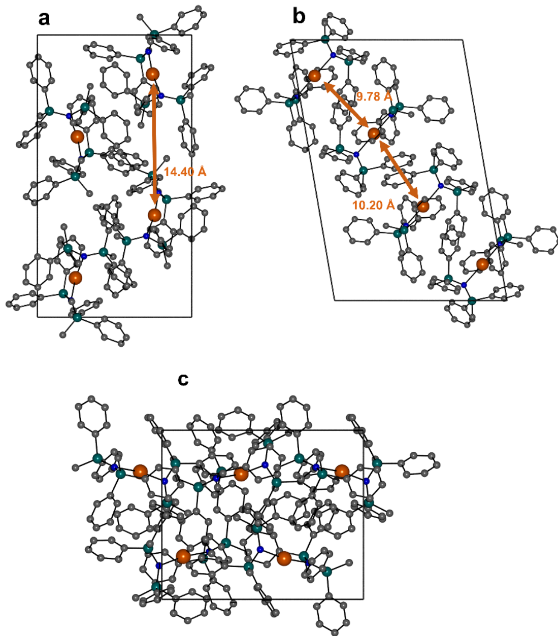
Supplementary Figure 1. Unit cell packing diagrams along the a-, b- and c-axis of \text{Eu}\{\text{N}(\text{SiMePh}_2)_2\}_2 (1).
