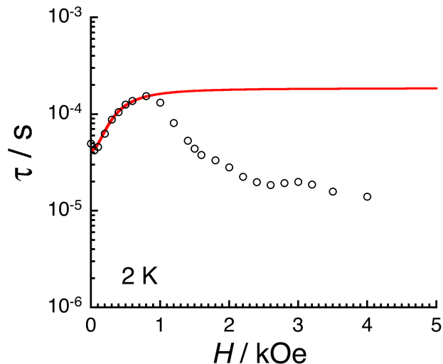
Supplementary Figure 11. Field dependence of the average relaxation times ( \tau ) between 0 and 4 kOe at 2 K determined from the generalized Debye fit of the frequency dependence of the in-phase ( \chi' ) and out-of-phase ( \chi'' ) components of the ac susceptibility (Supplementary Figure 9). The red line represents the best-fit to QTM relaxation, with parameters B_1 = 1.8(1) 10^4 \text{ s}^{-1} , B_2 = 22.8(2.3) \text{ kOe}^{-2} (Equations 1 & 2 without Raman term, and with the Orbach term set as a constant).
