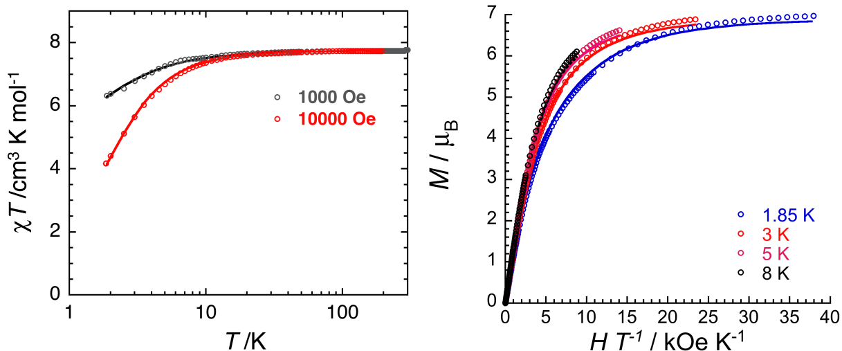
Supplementary Figure 8. Attempted fit of the experimental \chi T versus T (left) and M versus H (right) data to a S = 7/2 approximation with the following spin Hamiltonian: H = DS_{T,z}^2 , calculated with the software PHI. 1
