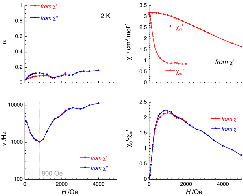
Supplementary Figure 10. Field dependence of the fitting parameters \alpha , \nu , \chi_0 , \chi_\infty , and \chi_0 - \chi_\infty , between 0 and 5 kOe at 2 K determined from the generalized Debye fit of the frequency dependence of the in-phase ( \chi' ) and out-of-phase ( \chi'' ) components of the ac susceptibility (Supplementary Figure 9).
