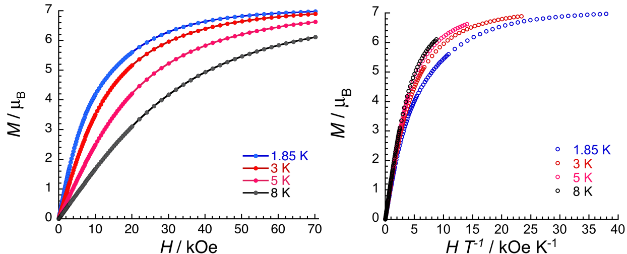
Supplementary Figure 7. Field dependence of the magnetization shown as M versus H (left) and M versus H/T (right) plots for \text{Eu}\{\text{N}(\text{SiMePh}_2)_2\}_2 ( 1 ) below 8 K.
