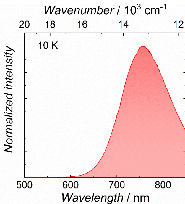
Supplementary Figure 5. Emission spectra for the crude oxidized product of \text{Eu}\{\text{N}(\text{SiMePh}_2)_2\}_2 ( 1 ) obtained in \text{C}_6\text{H}_5\text{F} ( \lambda_{\text{ex}} = 270 \text{ nm} ).
