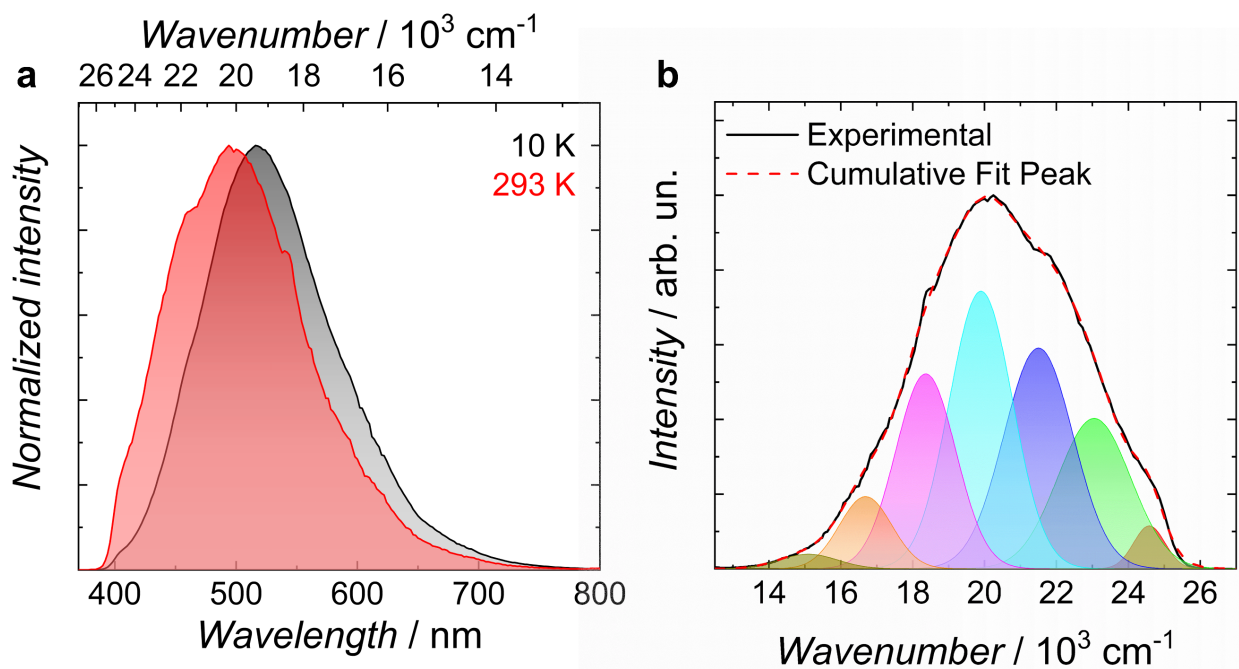
Supplementary Figure 3. (a) Emission spectra for 1 obtained at 10 and 293 K ( \lambda_{\text{ex}} = 270 nm). (b) Deconvolution of the 293 K emission spectrum.
