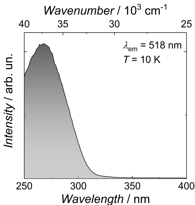
Supplementary Figure 2. Excitation spectrum for \text{Eu}\{\text{N}(\text{SiMePh}_2)_2\}_2 ( 1 ) obtained at 10 K ( \lambda_{\text{em}} = 518 nm).
