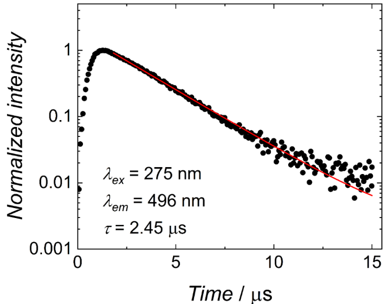
Supplementary Figure 4. Room-temperature emission decay (black points) and mono exponential function fit (red line) for \text{Eu}\{\text{N}(\text{SiMePh}_2)_2\}_2 ( 1 ).
