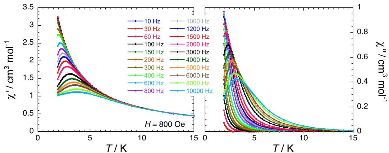
Supplementary Figure 12. Temperature dependence of the in-phase ( \chi' ; left) and out-of-phase ( \chi'' ; right) components of the ac susceptibility for \text{Eu}\{\text{N}(\text{SiMePh}_2)_2\}_2(\mathbf{1}) between 10 Hz and 10 kHz for the temperature range 1.9-15 K under an applied static field of 800 Oe.
