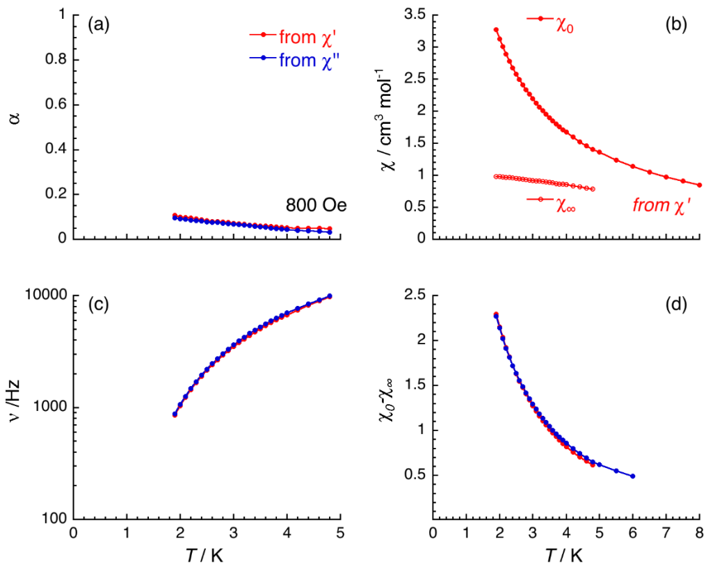
Supplementary Figure 14. Temperature dependence of the fitting parameters \alpha , \nu , \chi_0 , \chi_\infty , and \chi_0\chi_\infty , between 1.9 and 8 K under an applied static field of 800 Oe determined from the generalized Debye fits of the frequency dependence of the in-phase ( \chi' ) and out-of-phase ( \chi'' ) components of the ac susceptibility (Supplementary Figure 13).
