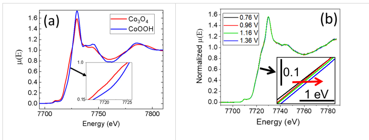
Figure 2: (a) Normalized XANES spectra recorded in air of typical CoOOH (blue curve) and \text{Co}_3\text{O}_4 (red curve) deposits on Au(111). The inset shows the edge region on an expanded energy scale. (b) Normalized XANES spectra of \text{Co}_3\text{O}_4 immersed in 0.1 M NaOH at different potentials. The inset shows a zoom in the edge region and the red arrow indicates the edge shift as a function of potential.
