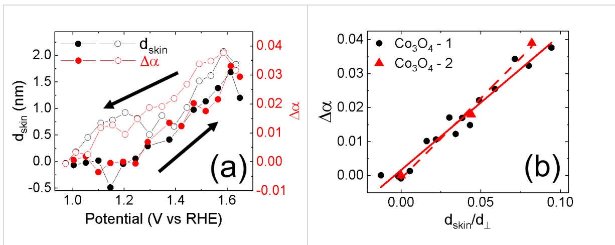
Figure 4: (a) experimental change of d_{skin}(U) (left y axis and black symbols) and the relative oxidation state \Delta\alpha(U) (right y axis and red symbols) as a function of potential between 0.97 and 1.67 \text{V}_{\text{RHE}} . (b) \Delta\alpha(U) as a function of the ratio d_{skin}(U)/d_{\perp} . The red lines are linear fits of the data for \text{Co}_3\text{O}_4 - 1 (solid line) and for \text{Co}_3\text{O}_4 - 2 (dashed line).
