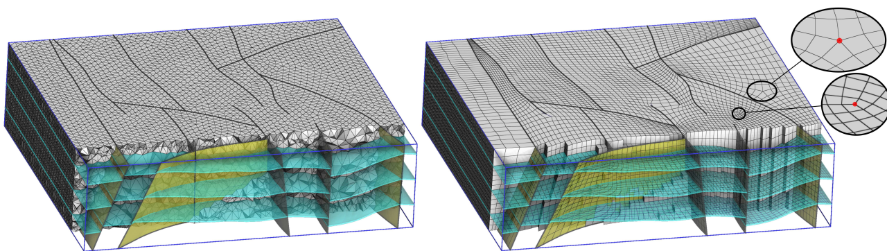
Figure 1: Given a geological model (left), our method automatically generates a full hexahedral mesh aligned with faults and horizons (right) at the cost of singular edges (close-ups).
