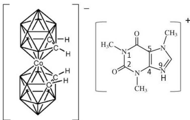
Figure 1. Molecular structure of [o\text{-COSAN}]^-/\text{caffeine} ion-pair complex
