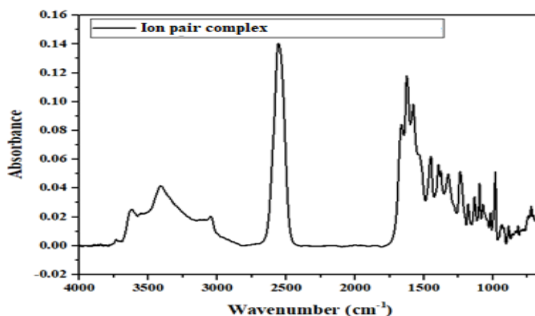
Figure 3. FTIR spectrum of the [o-COSAN] - /caffeine ion pair complex
