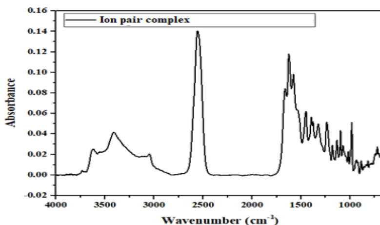
Figure 3. FTIR spectrum of the [o-COSAN] - /caffeine ion pair complex
