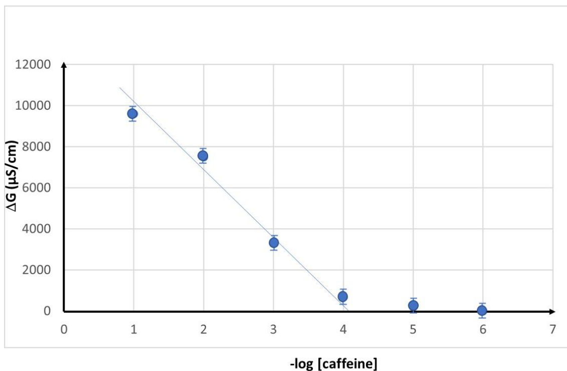
Figure 5. Calibration curve of the caffeine microsensor. Measuring conditions : differential mode, 10^{-3} M PBS buffer, pH 2.5
