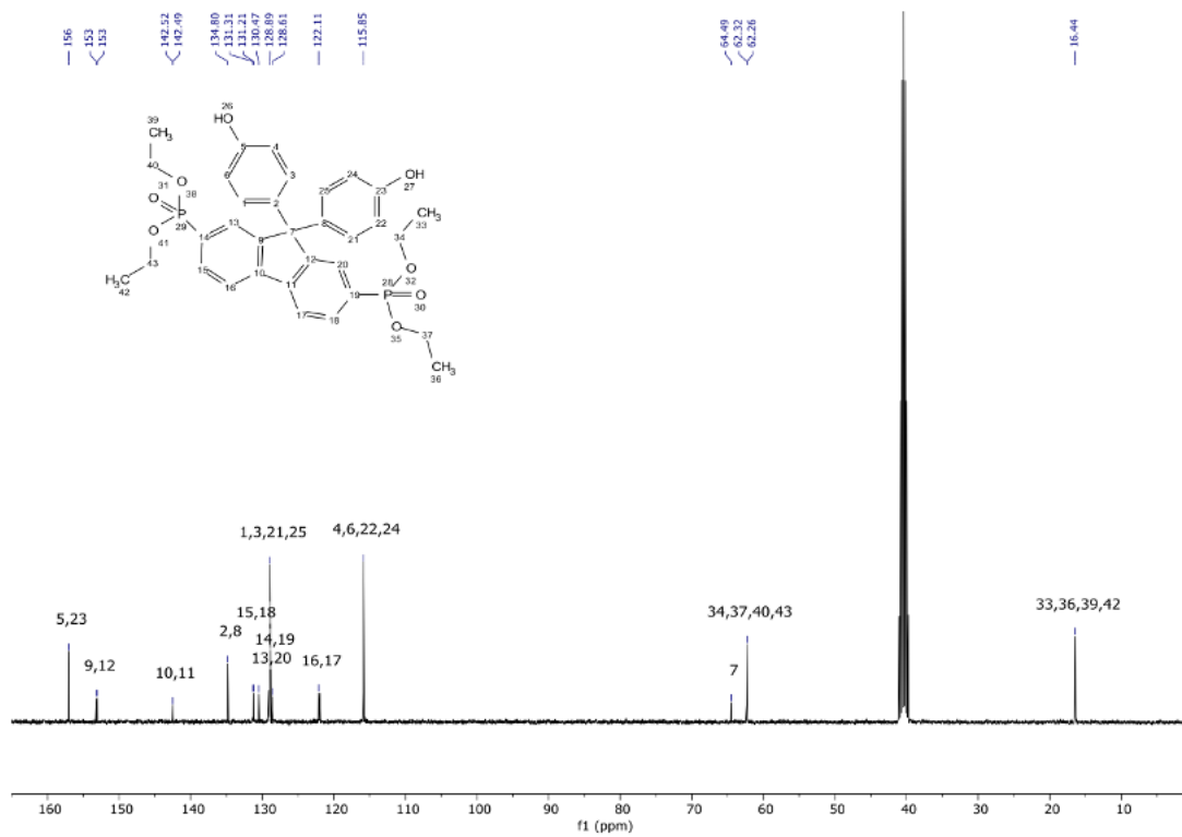
Figure S4. 13 C NMR (DMSO- d 6 , 80°C) of 2
