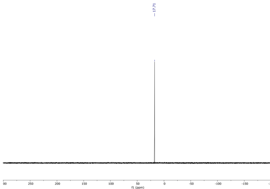
Figure S5. 31 P NMR (DMSO- d 6 , 80°C) of 2
