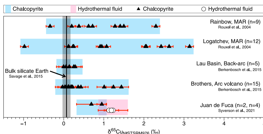
Figure 1. Overview of the copper isotope signatures measured in chalcopyrite and hydrothermal fluids collected in different geological settings, from mid-ocean ridges (MAR = Mid-Atlantic Ridge, Juan de Fuca) to arc and back-arc systems (Lau Basin and Brothers volcano). Data from Berkenbosch et al. (2015), Rouxel et al. (2004), Savage et al. (2015), and Syverson et al. (2021).
