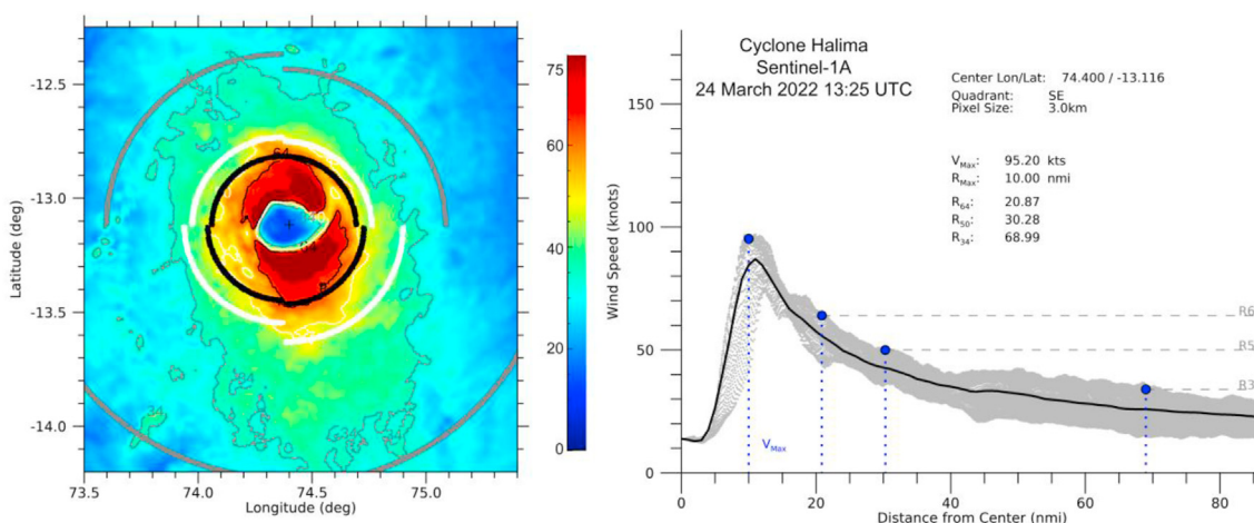
Fig. 1. SAR-derived wind speed map (left) for Cyclone Halima on 24 March 2022 from Sentinel-1A, from the NOAA SAROPS webpage (appendix C). The black, white and grey curves represent the derived fixes for the storm. Wind speed profiles (right) for the Southeast quadrant. Grey dots represent SAR-derived 3 × 3 km wind speeds in the quadrant and the solid back line represents the average wind speed at each distance from the storm's center. The blue dots are the radii of the (64/ 50/34 kt) fixes along the radial profile and correspond to the quarter circle locations shown in the left-hand plot. They are located at the 95 % percentile of the particular fixes wind speed.
