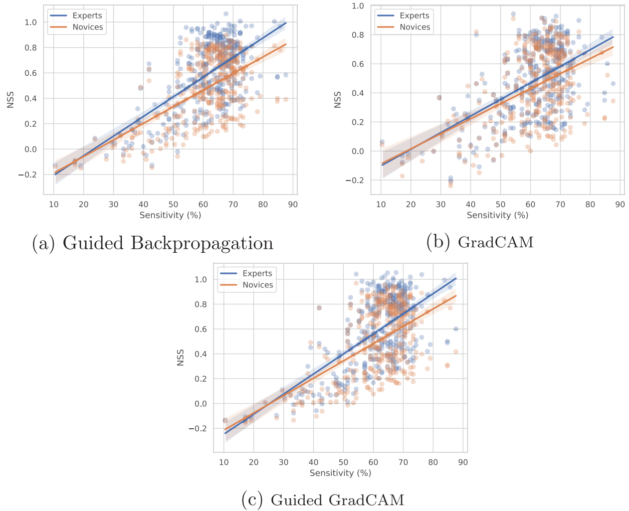
Figure E2. Comparison between artificial attention and human attention as a function of the network sensitivity. Artificial attention is obtained with three different post hoc methods: guided back-propagation, GradCAM, and guided GradCAM on three different networks on ResNet34. Results with VGG16 and VGG19 are similar.
