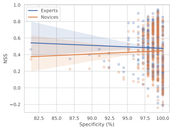
(b) GradCAM
