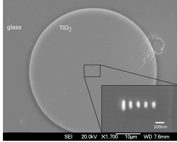
Figure 4. SEM image of Yagi-Uda gold nanoantenna centered on \text{TiO}_2 50 \mu\text{m} diameter microdisk planar waveguide. L_f=90 nm, L_d=85 nm, L_r=100 nm, y_r=85 nm and y_d=90 nm.
