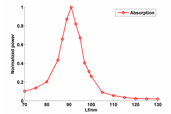
Figure 2. Normalized absorption power of single nanorod on a 80 nm \text{TiO}_2 slab, as a function of the rod length. The rod is excited by a dipole located 5 nm from its extremity.
