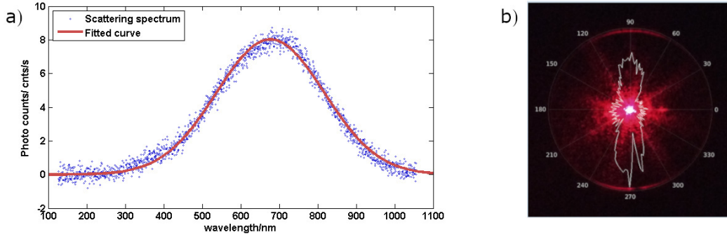
Figure 5. a) Dark field spectrum. Spectrum is fitted by Gaussian to estimate the resonance peak. b) Directional light coupling in \text{TiO}_2 waveguide through Yagi-Uda antenna when excited as a whole with a 670 nm laser light, polarized along the rod (x-axis). Red color is the wide field microscope image of light scattering and superimposed white line refers to the polar plot of the light scattered along the waveguide ring extremity. 0^\circ and 90^\circ refer to the antenna y-axis and rod x-axis respectively.
