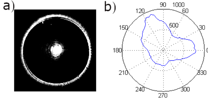
Figure 7. a) Image of scattering light of \text{TiO}_2 waveguide with Yagi-Uda antenna assisted QD emission. The inner spot is the light scattered by QD and Yagi-Uda antenna. The outer ring is the fluorescence light scattered from the edge of \text{TiO}_2 waveguide. b) Polar plot of the light scattered along the waveguide periphery.
