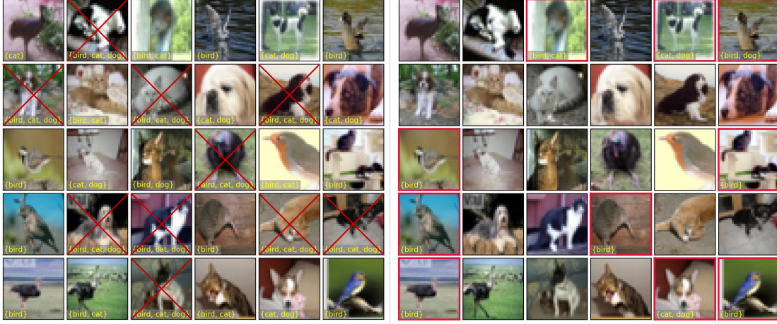
Fig. 1: Informative prediction sets in classification for CIFAR-10 dataset, restricted to the K = 3 classes “bird”, “cat”, and “dog” classes (iid setting). Informative prediction subsets are those of size smaller than K - 1 = 2 (i.e., non-trivial, Example 1.2 item 1). Selection by InfoSP are framed in red (right panel). \alpha = 10\% . See § 6 for more details.
