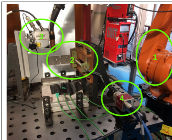
Figure 1 : WAAM equipment suited with acquisition systems.
