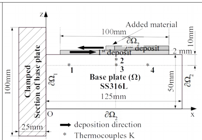
Figure 2 : schematization of base plate and overlaid deposits.
