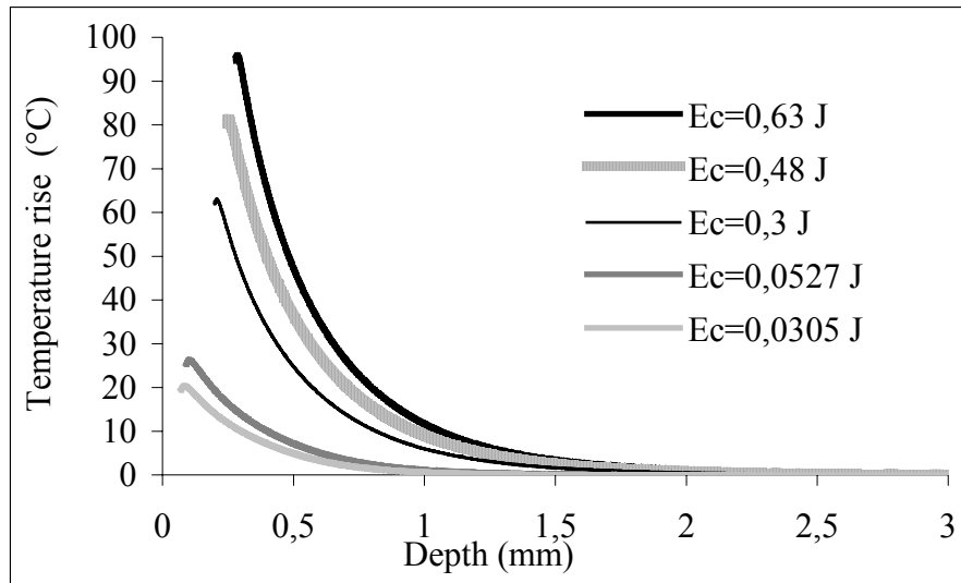
Figure 4: Increase in temperature as a function of the depth on the axis of symmetry of the system at the moment when the shot is at its maximal level of penetration. The radius of the shot is 3 mm. The respective energies of the impacting shots are given in the caption.
