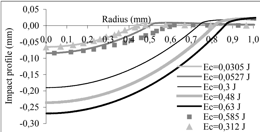
Figure 3: Impact profiles left on the surface after the impact. The diameter of the shot is 3 mm; the respective energies of the impacting shots are given in the caption. The lines correspond to numerical results while the marks correspond to experimental results.
