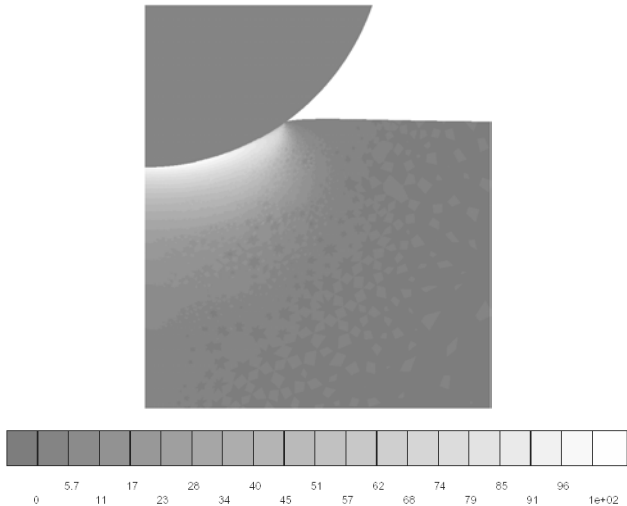
Figure 2: Field of the increase in temperature due to the impact of a shot of 3 mm in diameter on a steel massif. This field corresponds to the instant of maximal penetration of the shot. A quarter of the shot is shown on the figure for geometrical scaling, the temperature scale goes from 0 to 100 °C. The energy of the incident shot is 0.63 J.
