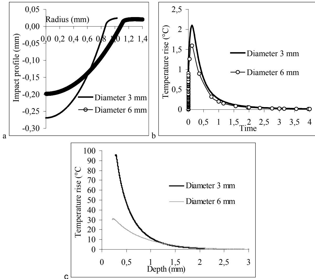
Figure 6: Comparison of various profiles for two shot diameters and the same energy for the impacting shot (0,63 J). a) Comparison of the impact profiles left on the surface. b) Increase in temperature as a function of time. The temperature is taken at a point located on the axis of symmetry of the system and at a depth of 2 mm; it is given as a function of time. The contact between the shot and the semi-infinite body starts at 1 \mu s, the maximal shot penetration is obtained at 1,8 \mu s then the shot is withdrawn and the computation stops at 4 s. c) Temperature increase as a function of the depth.
