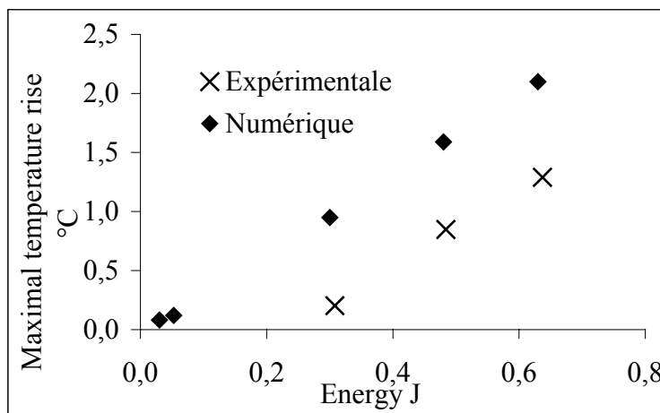
Figure 5: Maximal increase in temperature at a point of depth 2 mm as a function of the energy of the incident shot, comparison between experimental and numerical results for a shot of diameter 3 mm.
