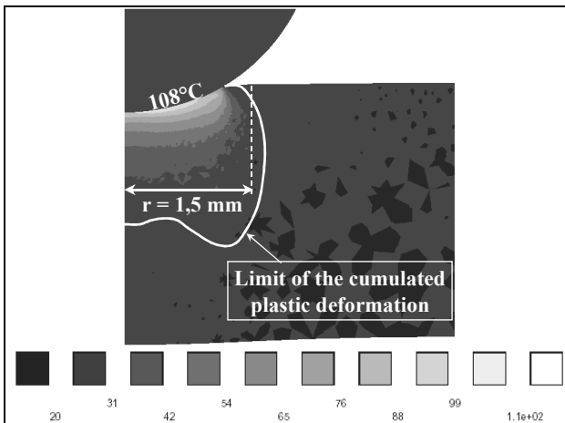
Figure 7: temperature field at the maximum penetration of the shot (~8 \mu s after the beginning of the impact), velocity 80 m/s.
