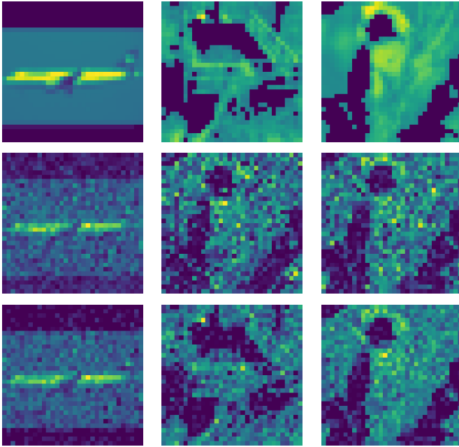
(b) Decomposed material maps. Top row: ground truth material map. Middle row: decomposition using the RU method. Bottom row: decomposition using the joint method.
