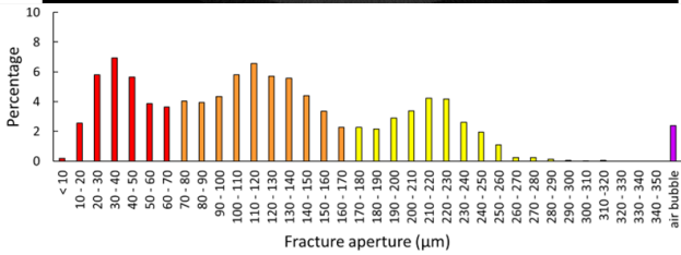
Figure 9: Fracture apertures of sample #16 obtained with XRCT. The distributions are displayed as probability density functions. Voxel size: 24.4 µm.
