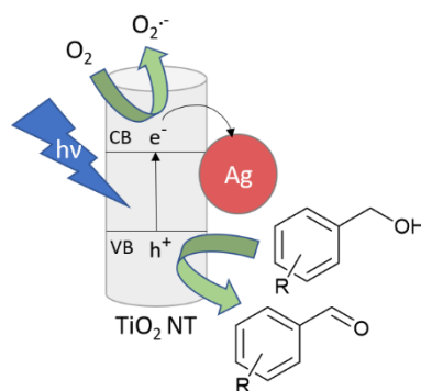
Scheme 2. General mechanism for the photocatalytic oxidation of benzyl alcohol with Ag-doped rutile nanotubes.
