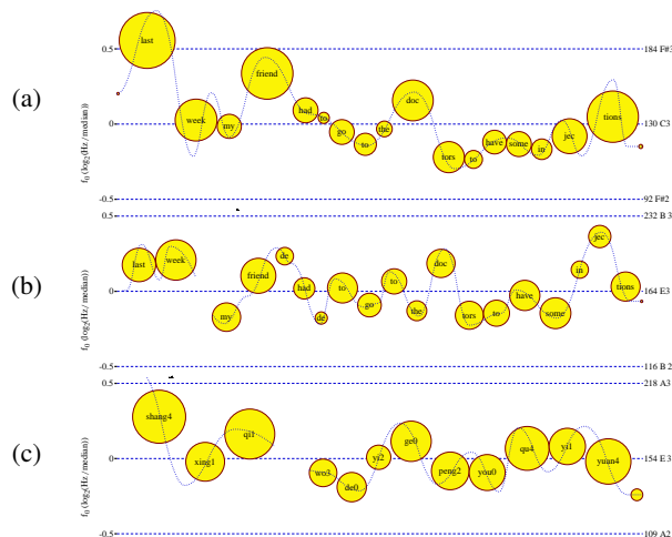
Figure 1: Prosody display of English (a), Chinese English (b) and Mandarin Chinese (c). Note: Though the Chinese speaker read the same English sentence as that in (a), two epentheses occurred, which resulted in two more syllables ( de ) in (b).
