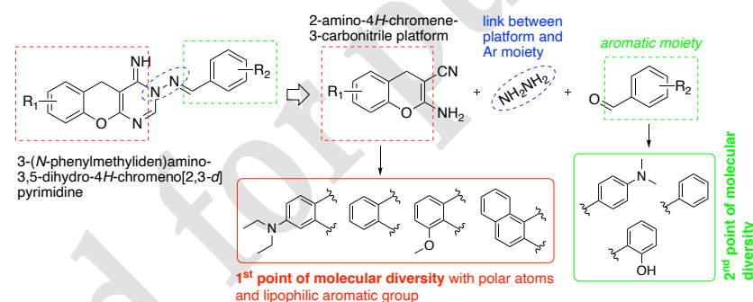
Figure 2. Retrosynthetic strategy towards 3-( N -phenylmethyliden)amino-4-imino-3,5-dihydro-4 H -chromeno[2,3- d ]pyrimidine and building blocks for the introduction of molecular diversity.
