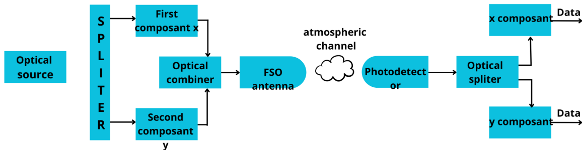
Fig. 2. PoSK Block diagram
