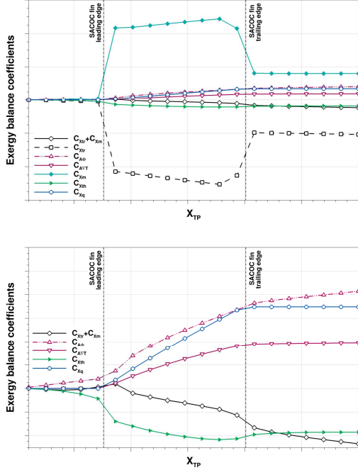
Figure 3: Overall evolution of the exergy balance for a variation of the control volume's downstream limit (top) and detail of specific components (bottom). Isolated SACOC fin case with aerothermal-coupling-based wall boundary condition.
