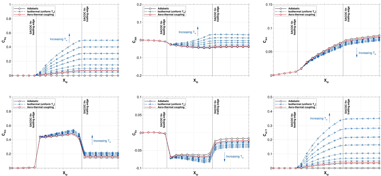
Figure 5: Impact of different boundary conditions (adiabatic wall, isothermal wall at varying uniform wall temperature values, aero-thermal coupling) on components of the exergy balance for the isolated SACOC fin case. The coefficients are adimensionalised by a common reference surface.
