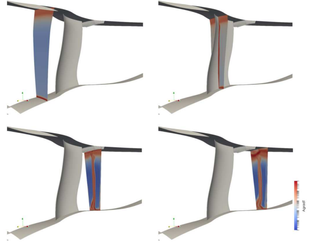
Figure 12: Thermal energy generation at different axial positions in the OGV-SACOC region of the fan-OGV-SACOC-BPD configuration.
