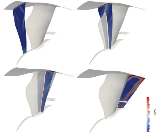
Figure 13: Viscous anergy generation at different axial positions in the fan region of the fan-OGV-SACOC-BPD configuration.
